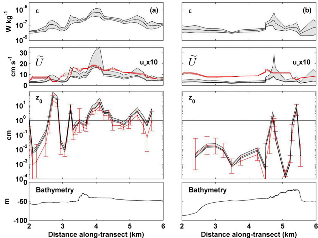
FIG. 14. Near-bottom TKE dissipation rate \varepsilon , near-bottom velocity \tilde{U} , friction velocity u_* ( \times 10 ), roughness length z_0 , and bathymetry at transects (a) T1 and (b) T2. The shaded regions in the first three panels are the 95th percentile errors for each parameter. For z_0 , both the value calculated using only the near-bottom velocity (black line) and the mean and standard deviation of the three z_0 values obtained using \tilde{U}_1 and \tilde{U}_2 (red line with error bars) are shown. The horizontal line is at 1 cm, the lowest reported value for coral roughness in prior studies (Rosman and Hench 2011).
