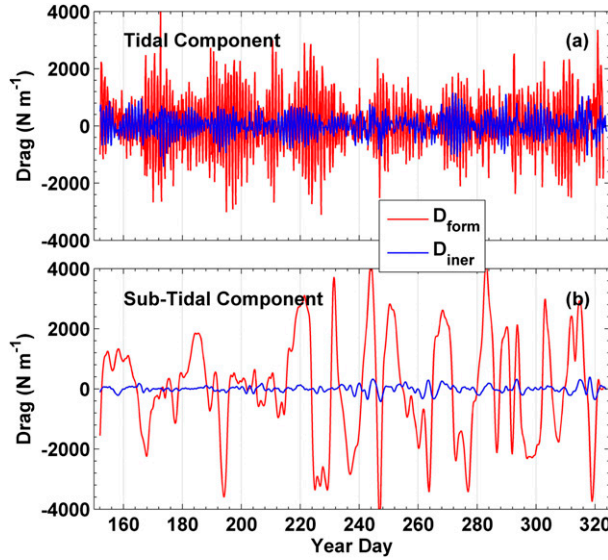
FIG. 9. Total form drag D_{\text{form}} based on interpolated pressure fluctuations (method II). (a) Tidal band and (b) subtidal bands (period > 2 days). The blue line in (a) and (b) is the inertial component of the form drag D_{\text{iner}} due to acceleration/deceleration of the flow.
