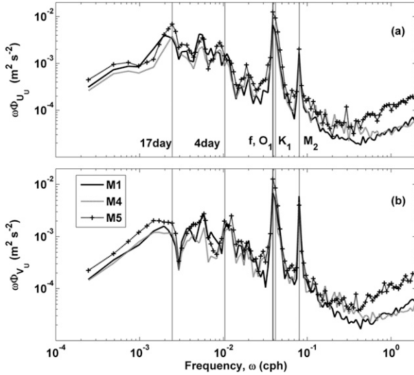
FIG. 4. Depth-averaged frequency-weighted velocity spectra in the upper 50 m based on time series of velocity shown in Figs. 3a and 3b. (a) U and (b) V . Spectra at M1, M4, and M5 are plotted. The vertical lines denote frequencies of M2, K1, O1, f (inertial), 4-day, and 17-day motions.
