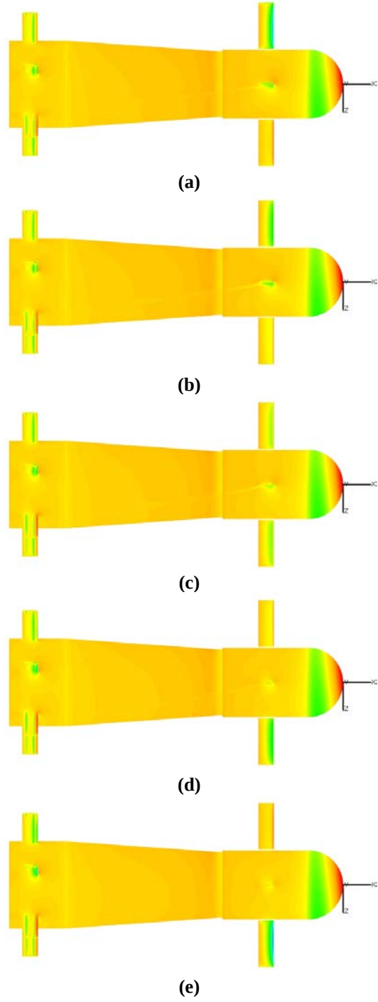
Figure 6. Computed surface pressure contours at \alpha = -5^\circ and roll = 0^\circ for different canard deflections, (a) -8^\circ , (b) -4^\circ , (c) 0^\circ , (d) 4^\circ , and (e) 8^\circ . ( 5.0e + 04 \leq P \leq 1.0e + 05 Pa).
