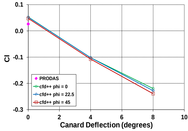
Figure 9. Computed roll moment coefficient, \alpha = -5^\circ .
