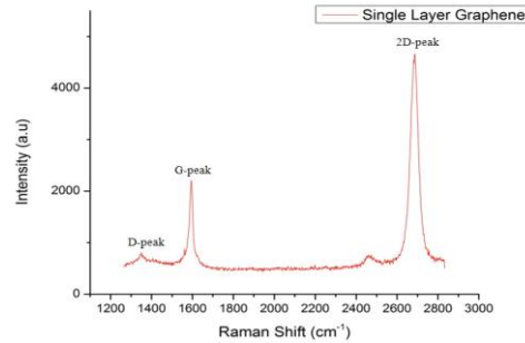
Fig. 3. Raman spectrum of CVD graphene.
