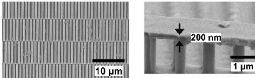
Fig.12. TEM cross sectional membrane produced by reactive ion etching. Left: Top view of patterned membranes in a bulk single crystal diamond. Right: membranes mechanically removed from the parent crystal and transferred onto silicon spacer posts.
