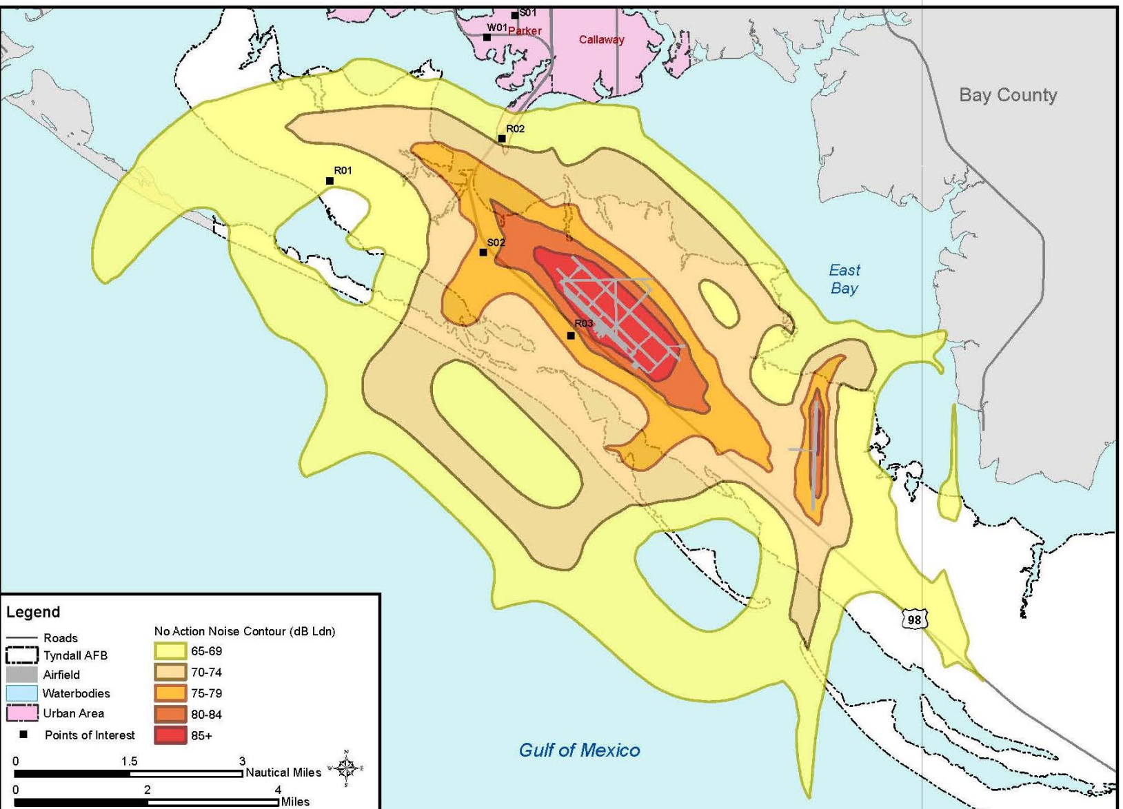
Figure 4-3. Noise Contours under the No Action Alternative and Baseline Conditions
