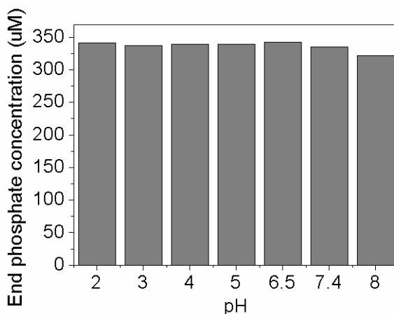
Figure 3. Stability of polyP at 37 °C and various pH conditions.
