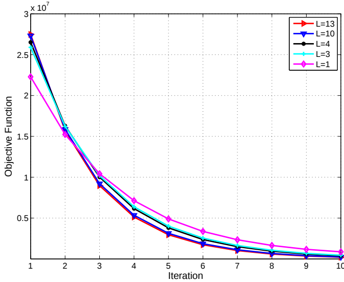
Fig. 8. The objective function value as a function of iteration number for the experiments with a Cameraman image with various number of looks.
