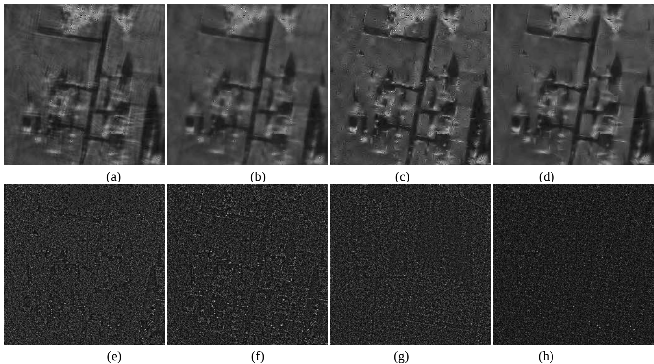
Fig. 11. Despeckled images. Restored using (a) the SBT method, (b) the MCA method, (c) wavelet-based thresholding and (d) our method. (e)-(h) are the noise images corresponding to the filtered images in (a)-(d), respectively.
