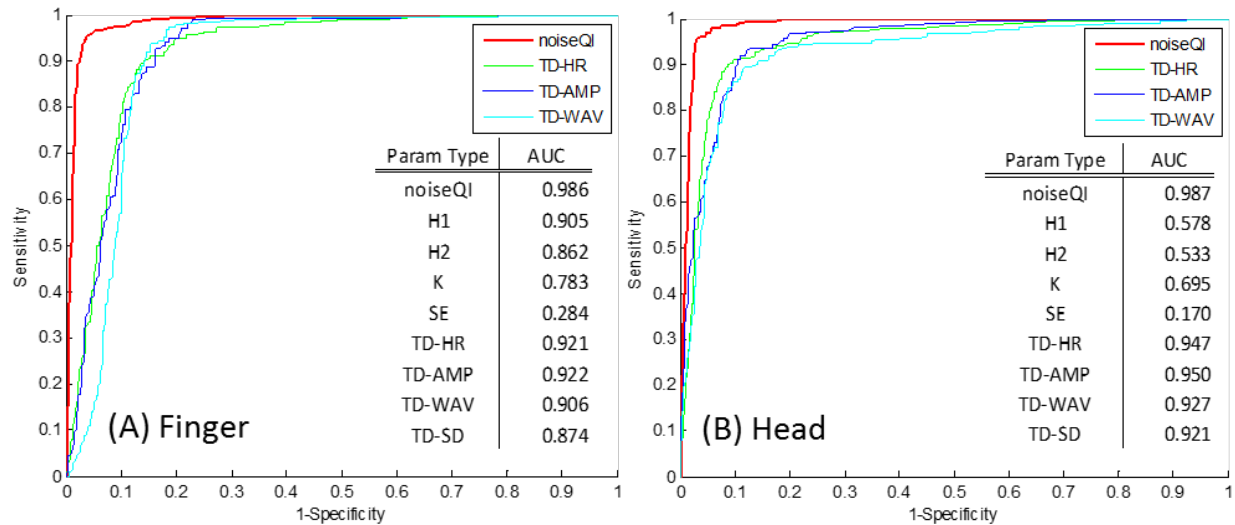
Figure 7. Receiver-operating-curves (ROCs) of all the features used in MNA detection algorithms: Our proposed VFCDM (noiseQI); Hjorth parameters (H1,H2); Statistical features (K,SE), Time-domain features (TD-HR, TD-AMP,TD-WAV,TD-SD). (A) Finger data; (B) Forehead data.
