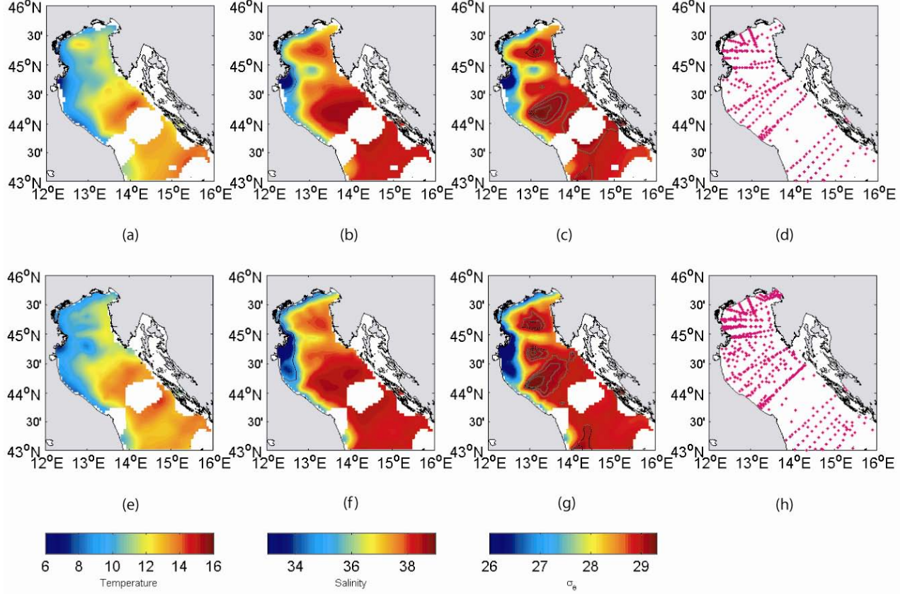
Figure 5. Climatological surface temperature, salinity and density maps during Bora events (top row) and for the overall wintertime mean (bottom row). Charts in the rightmost column indicate data distribution. The Bora climatology (top row) and, to a lesser degree, the winter maps (bottom row) reveal two distinct dense water pools in the Northern Adriatic separated by a filament of fresh, cold water.
