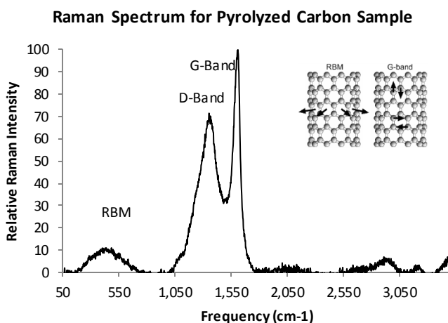
Figure 6: Raman spectrum of pyrolyzed carbon sample, showing graphite-related (G-band), defect-induced (D-band), and Radial Breathing Mode (RBM). Inset: diagram of RBM and G-band.
