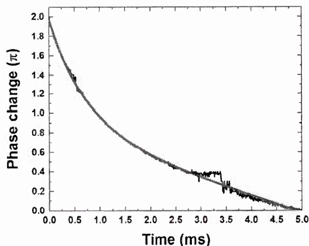
Fig. 11: Measured phase decay time of the PNLC sample. Black line is experimental data and red line is fitting with Eq. (7) and \varphi_0 = 2\pi .
