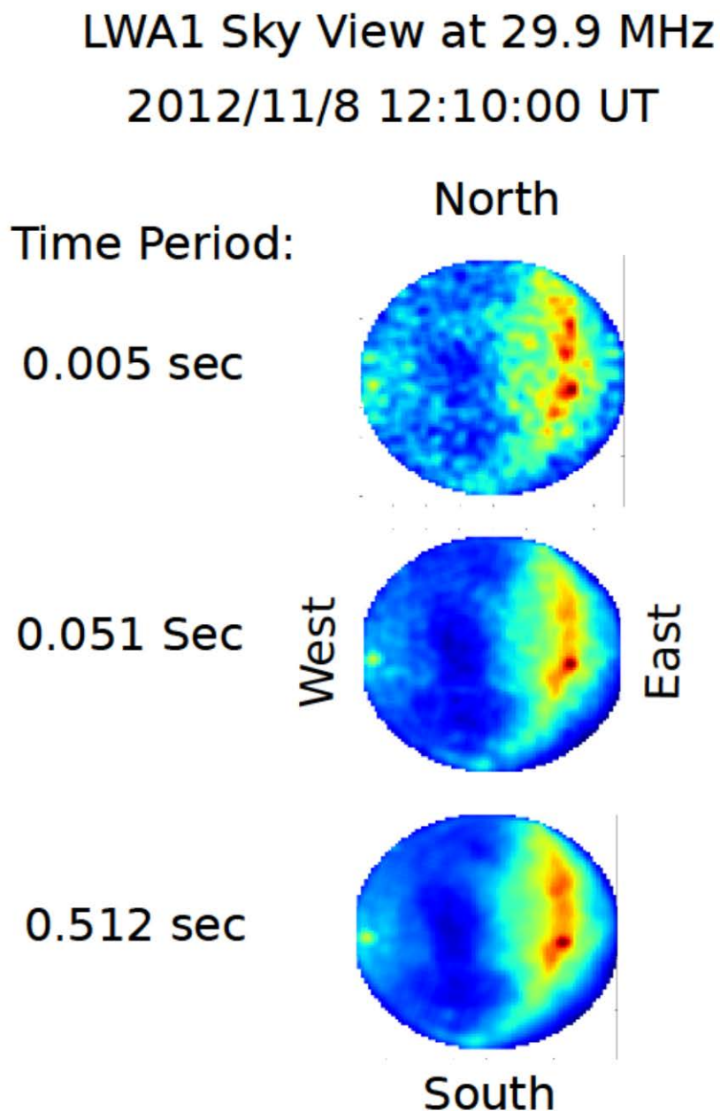
Figure 3. LWA 1 Sky view at three time resolutions during the Kirtland Digisonde operation.
