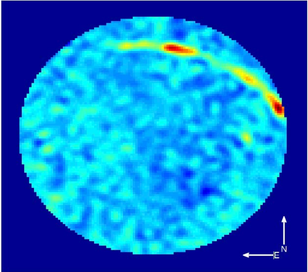
Figure 10. Image of the sky, after subtraction, of the fireball of January 21, 2014 which covered 92^\circ . The edge of the circle marks a cutoff of 25^\circ above the horizon.
