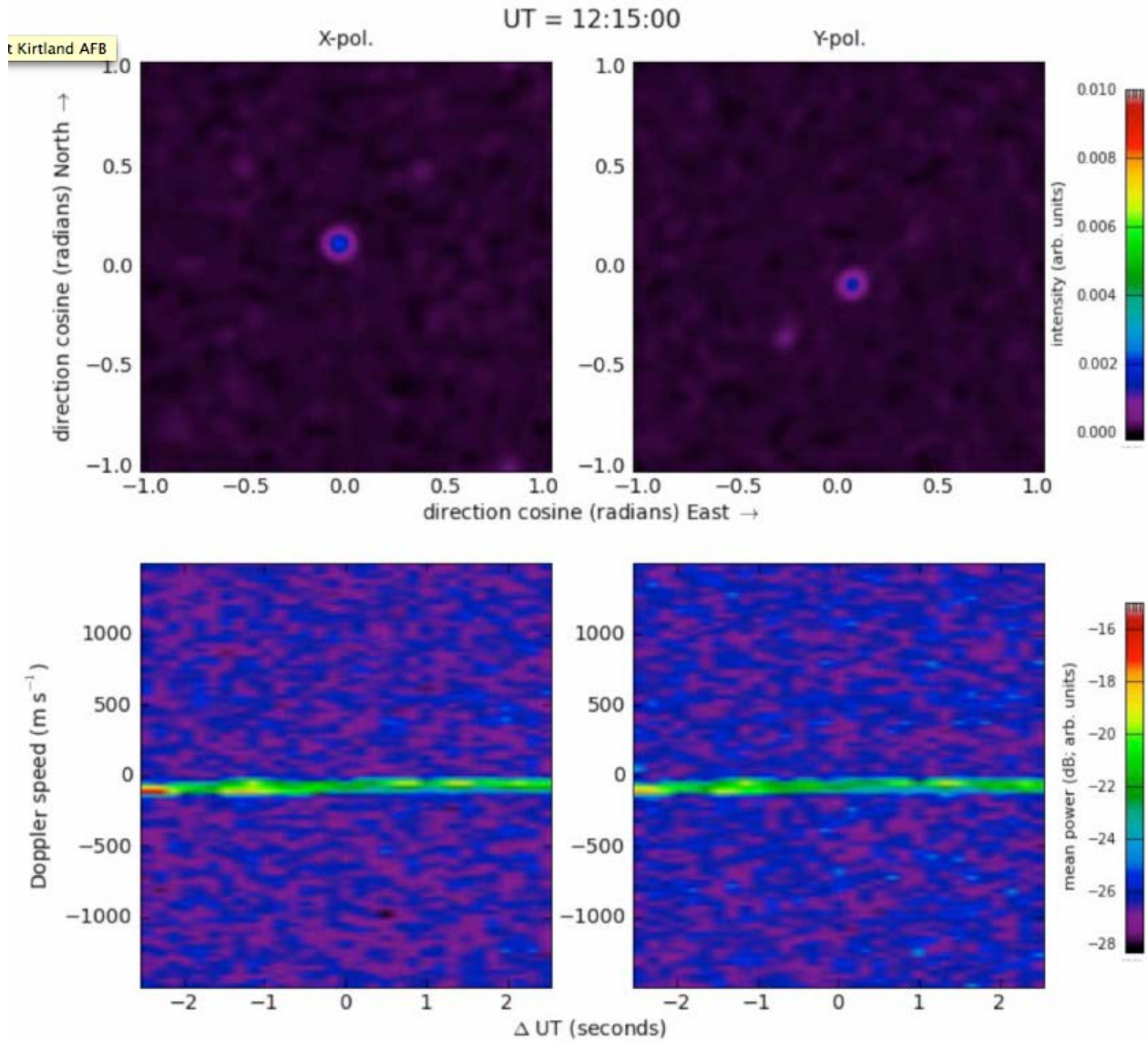
Figure 9. Detection of echoes from the Kirtland Digisonde off of meteor trails with LWA1.
