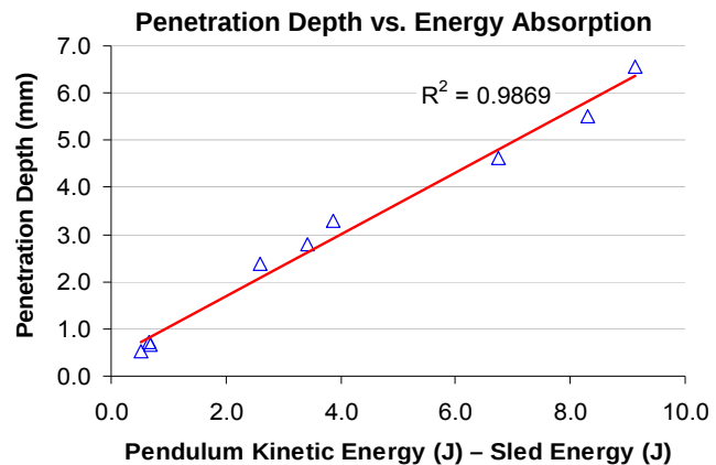
Figure 2: Relationship of the depth of polyurethane foam penetration vs. the energy absorption measure (difference between the pendulum kinetic energy and sled energy values).
