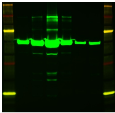
Figure 3: Western blot of pure CYP27B1 fractions.
