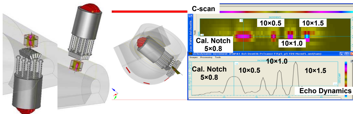
Figure 22. Example of Flexible Matrix Phased Array Applied on Radius Features
