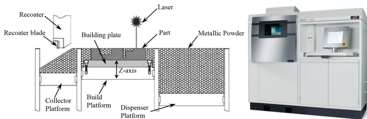
Figure 5. Schematic of Laser Powder-Bed Fusion (L-PBF) Process (left); EOSINT M280 Machine (right)
