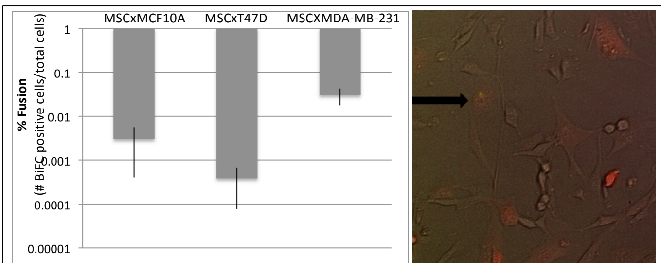
Figure 1. Spontaneous fusion of human mesenchymal stem cells with either human breast epithelium (MCF10A), weakly metastatic breast tumor line (T47D) or highly metastatic breast tumor line (MDA-MB-231). Mesenchymal stem cells were transfected with BiFC half VN-H3.1 and breast epithelium or breast tumor lines were transfected with BiFC half YC-H3.1 via lentivirus. Twenty four hours after transfection, cocultures were initiated and cultures were monitored for fluorescent signal indicative of cell fusion. The number of fluorescent cells was determined for each coculture and reported as a percentage of the total number of cells per well. n = 6 wells from 3 separate experiments. Error bars = standard deviation. Image to the right shows a fusion product (black arrow) formed between MCF10A and MSC. Note green fluorescence signal in nucleus indicative of BiFC pairing and therefore cell fusion. Red fluorescence indicates cells that have received one half of the BiFC pair.
