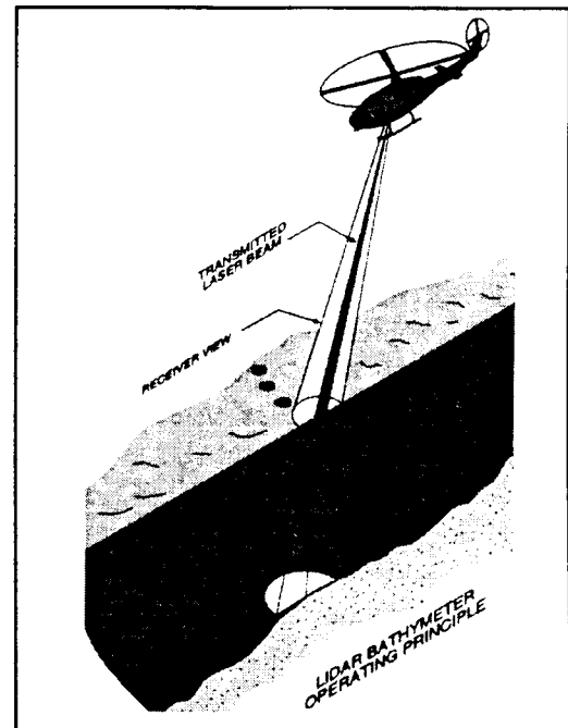
Figure 2. SHOALS operating principle, laser pulses at 200 Hz while being scanned 180 deg across the flight path of the helicopter
