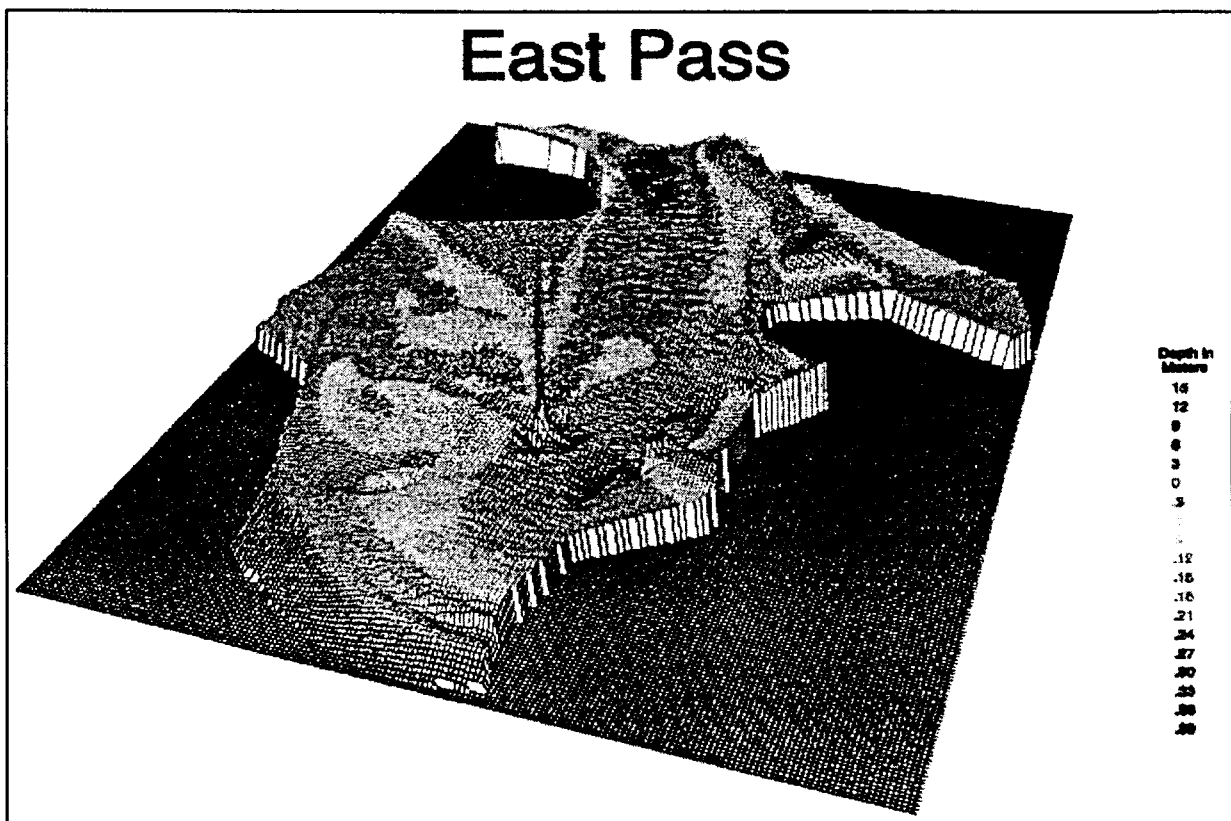
Figure 6. SHOALS survey of East Pass at Destin, Florida, after the passage of Hurricane Opal
