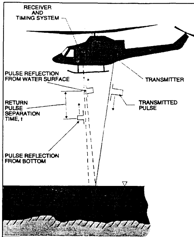
Figure 3. Lidar returns from the water surface and sea bottom. The time difference between the two returns indicates the depth
