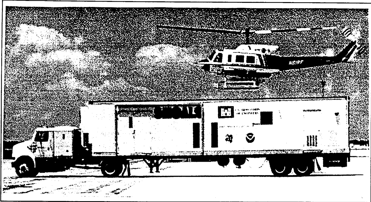
Figure 1. SHOALS Airborne lidar survey system. Capable of providing high resolution surveys of coastal projects
