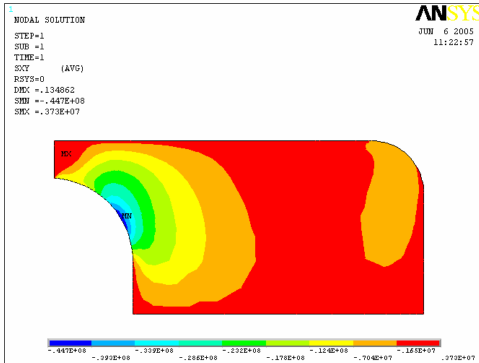
Figure 14 – Pusher plate stress in xy-axis for the discarding launch concept 1
