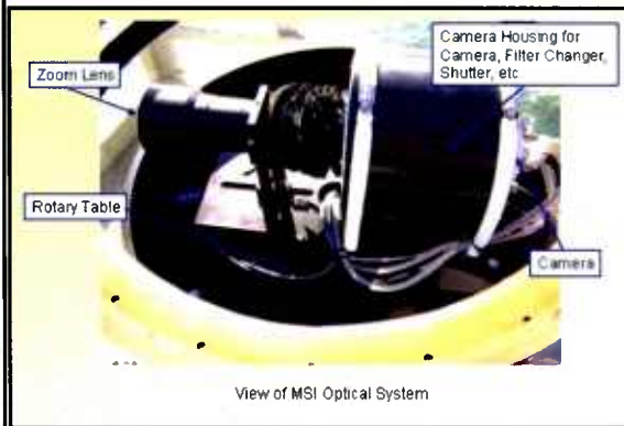
Fig. 6-5. MSI Optical System
