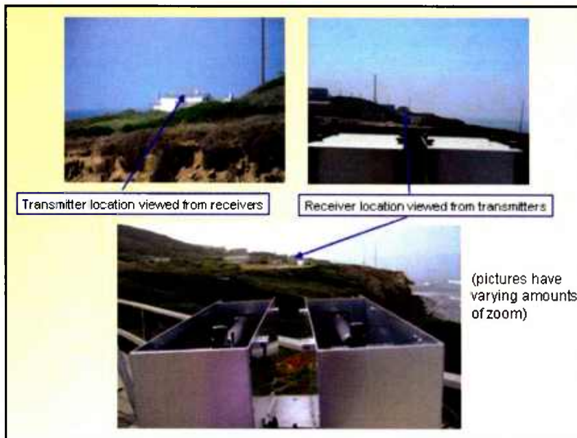
Fig. 6-11. Path of Sight for the two Transmissometers
