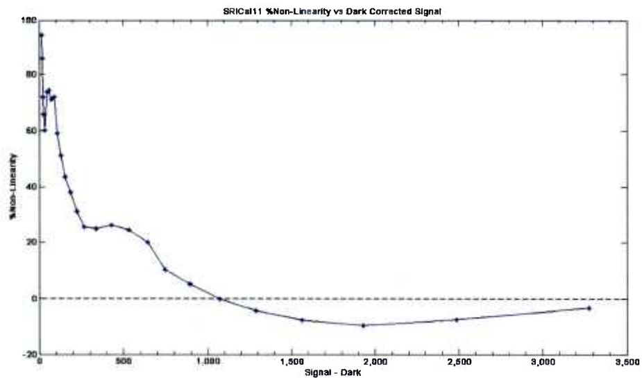
Fig. 8-3. Linearity calibration vs. radiance for Exposure 32,000 \mu sec, plot of % non-linearity vs. dark-corrected signal
