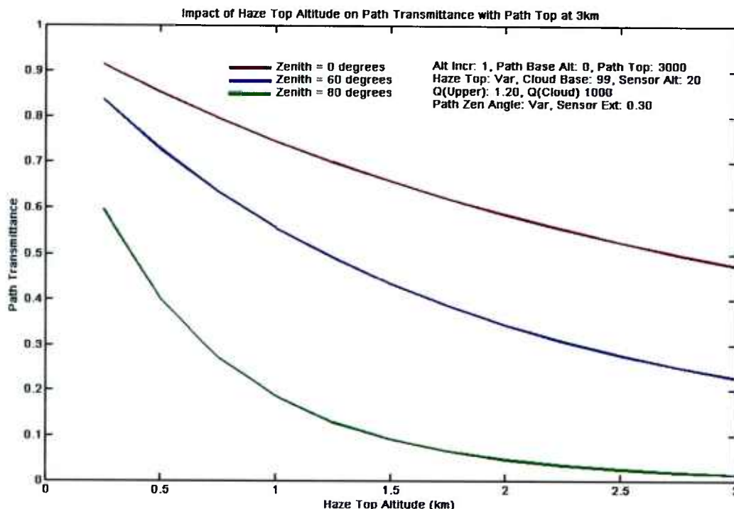
Fig. 11-8. Impact of varying Haze Top for a Path Top of 3 km and for Zenith Angles 0°, 60°, and 80°
