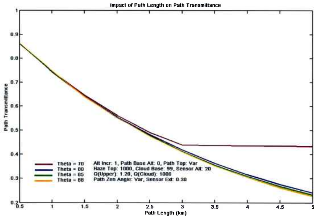
Fig. 11-7. Impact of varying Path Length for Zenith Angles 70°, 70°, 85° and 88°
