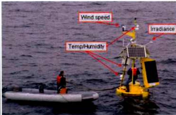
Fig. 6-9. Deployment of Flux Buoy
