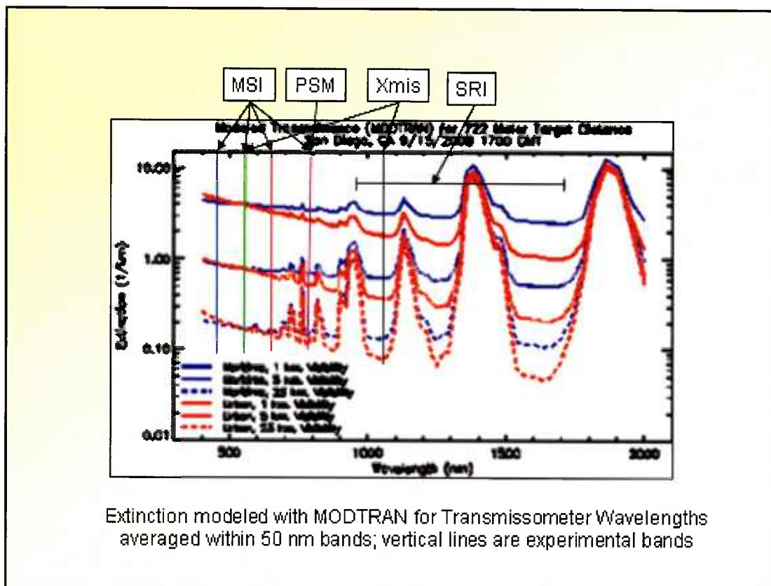
Fig. 5-2. Extinction Coefficients with the passbands of the instruments superimposed
