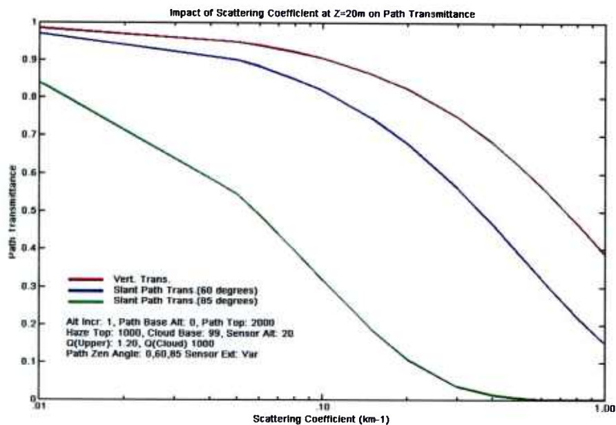
Fig. 11-2. Slant Path Transmittance as a function of extinction near the ground, for three paths, at look angles 0°, 60°, and 85°.
