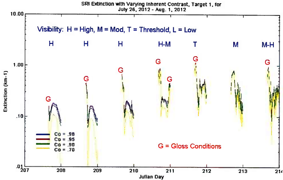
Fig. 8-13. Derived SWIR Extinction Coefficient for July 26 – Aug 1 2012 looking WNW at 300^{\circ} (T), using varied Inherent Contrast Values
