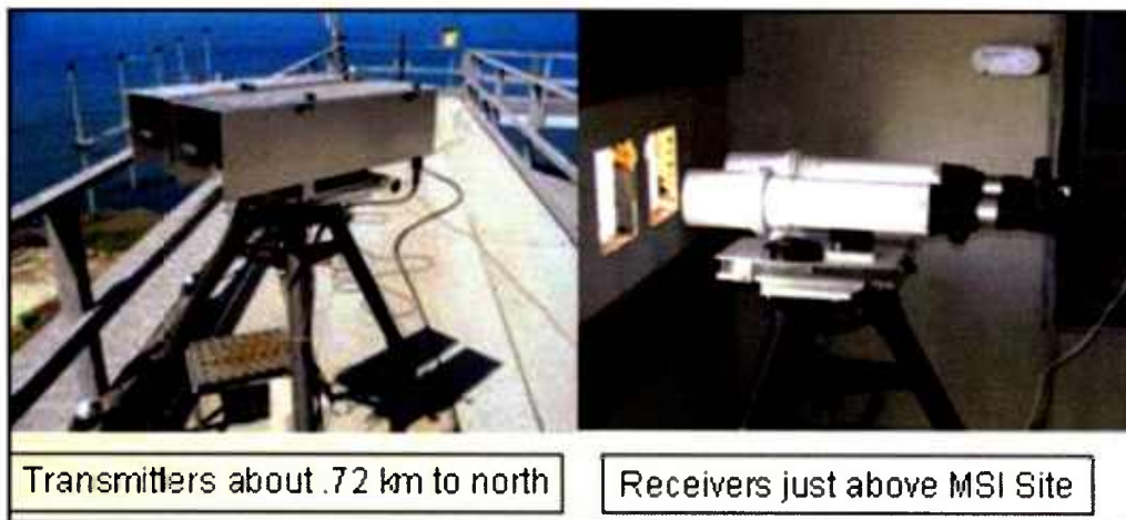
Fig. 6-12. Transmissometer Transmitters and Receivers
