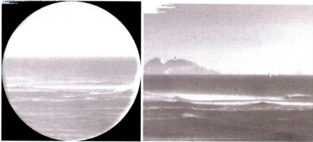
Fig. 9-9. MSI and SRI images, looking South at 180 ° (T), 14 Feb 2010 2300Z (1500 PST); Ext(MSI)=.272 \text{km}^{-1} , Ext(SRI)=.168 \text{km}^{-1} ; Ext(PSM)=1.12 \text{km}^{-1} ; Red V=11 km, SWIR V = 18 km, PSM V = 2.7 km
