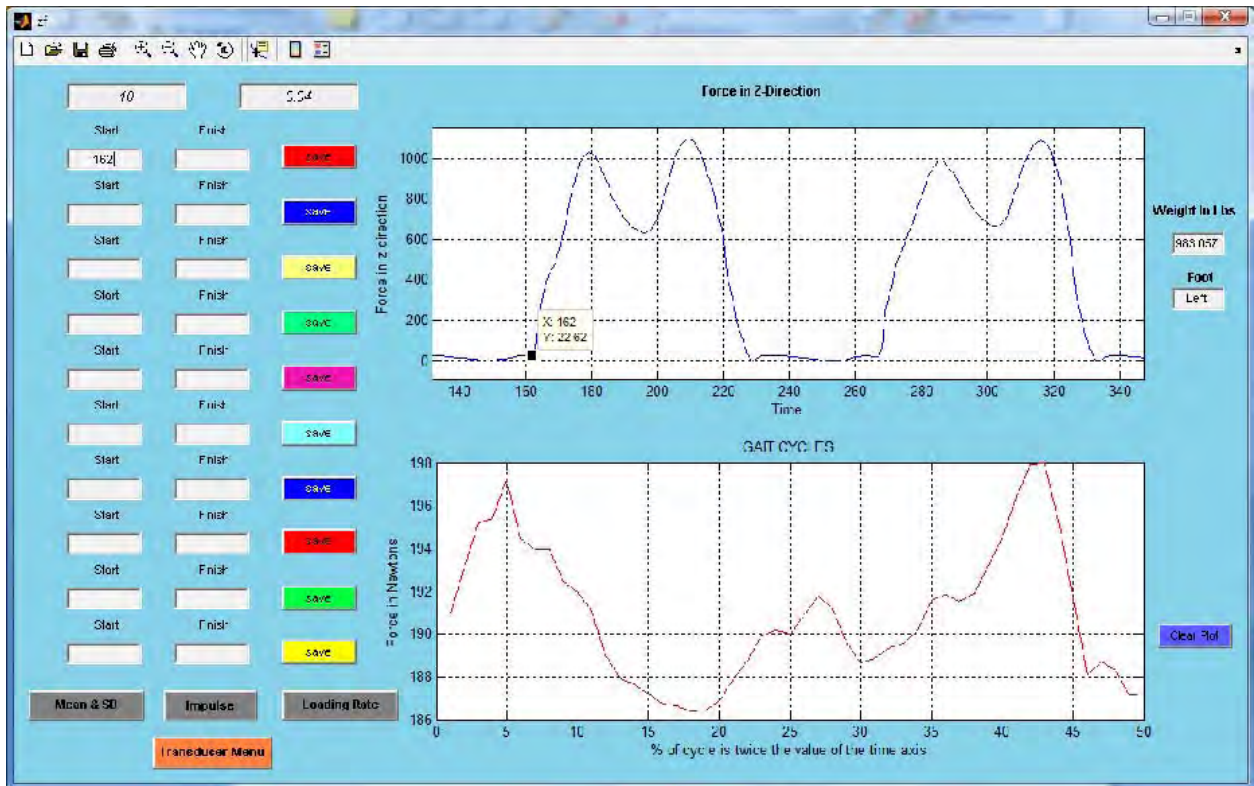
Figure 3-6. Identification of Points Representing Heel Strike
