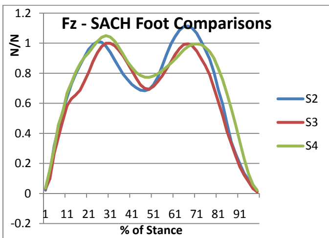
Figure 5-1. Normalized Forces and Moments for the SACH foot. An asterisk (*) indicates that the transducer data were multiplied by -1 to allow a comparison of left and right feet.
