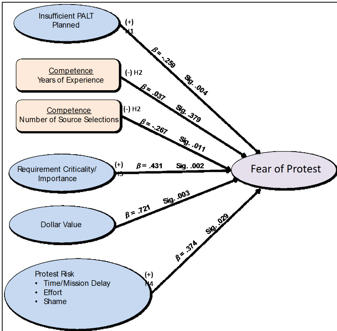
Figure 2. Left Side Hypothesized Model
