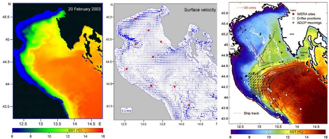
Figure 1. DieCAST-data comparison
