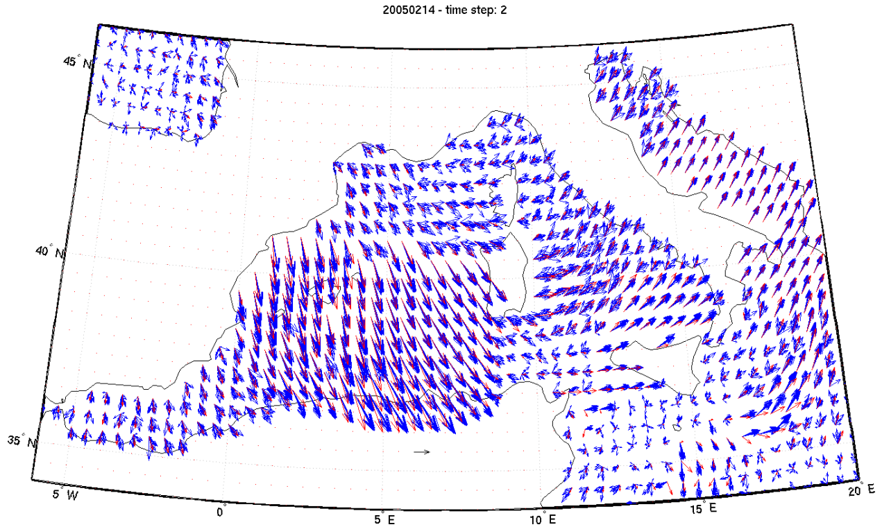
Figure 1. Surface vector wind field realizations for the western Mediterranean basin. Ten blue wind vectors are plotted at each MFS-Wind-BHM output grid location for this snapshot. A red vector at each location represents the surface wind analysis from ECMWF for this time. The reference vector at about 6°E, 36°N is scaled to 10 ms -1 . The snapshot corresponds to the penultimate ensemble forcing field during the data assimilation period for the reforecast experiment (day 14A). A low pressure system is deepening over Sardinia, and the Mistral winds are freshening to the west and southwest. Where wind speeds are large, the ensemble winds are more narrowly distributed about the ensemble mean wind. In sheltered regions (i.e. near the Sicily Strait), the wind speeds are low and direction uncertainty is larger. The ten realizations at each grid location are all consistent with the uncertainties expressed in the data stage distribution, based on ECMWF analysis and scatterometer observations, and with the process model stage distribution.
