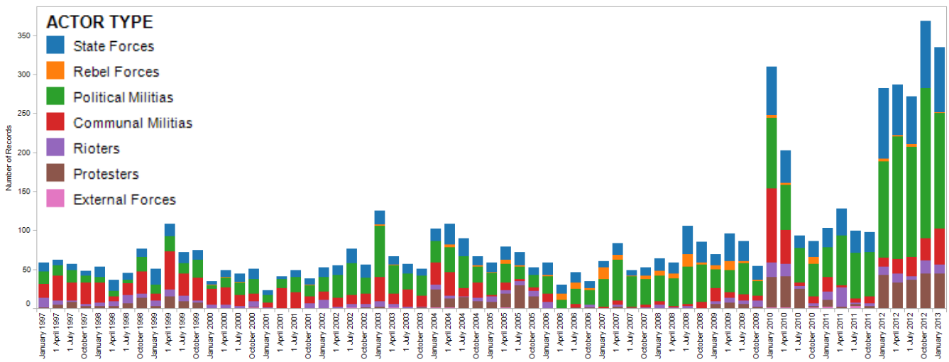
Figure 4: Conflict events by actor type, Nigeria, 1997 - March 2013.
