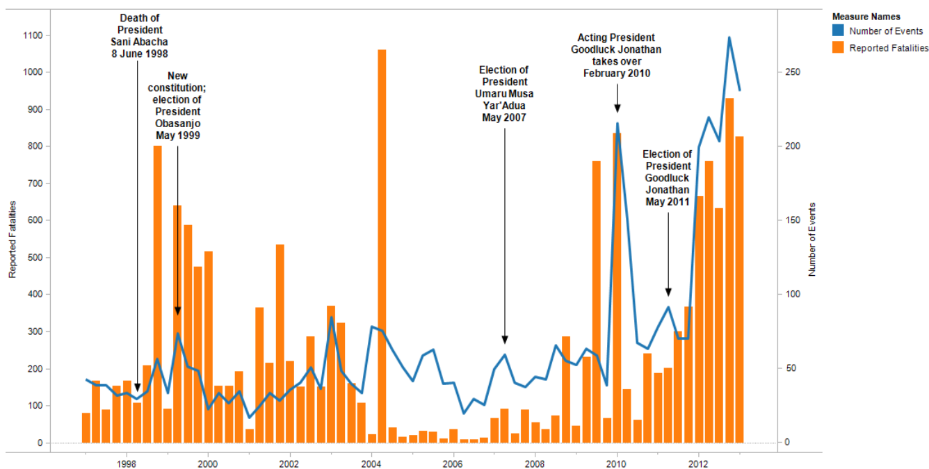
Figure 1: Conflict Events and Reported Fatalities, Nigeria, 1997 - March 2013.
