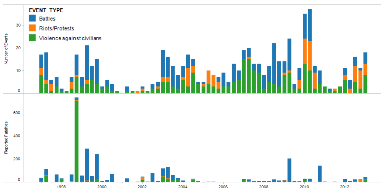
Figure 5: Conflict events and fatalities in Niger Delta region (Bayelsa, Cross River, and Delta), 1997 - March 2013.
