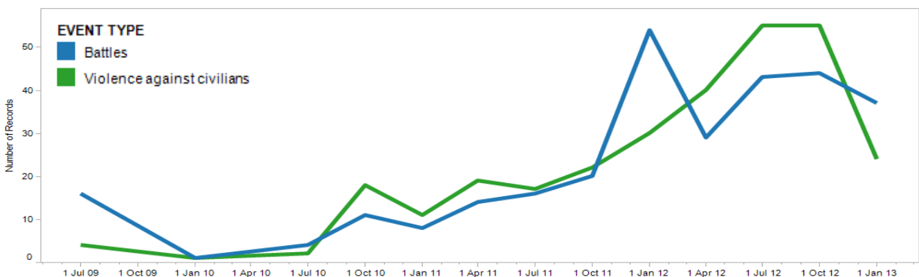
Figure 3: Boko Haram violent activity by type, 2009 - March 2013.
