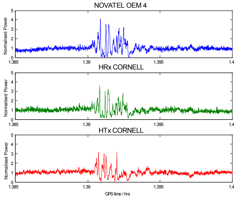
Figure 3. Example of GPS amplitude scintillations at high latitudes.
