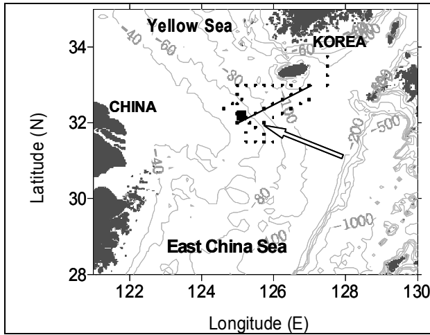
Fig. 4. Bottom topography of the northern East China Sea. CTD and Turbomap measurement sites (small circles) and ADCP/CTR7 moorings (large square) are indicated. The expected propagation of internal wave packets from the ocean shelf break is shown by the arrow.
