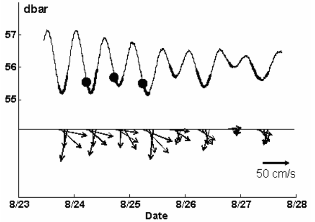
Fig. 5. A time series of the near-bottom pressure at the test site and the hourly-averaged current vectors for periods of low tide. The periods corresponding to the NLIW episodes are in bold. The cases where solitary waves preceded wave packets are shown by larger circles.
