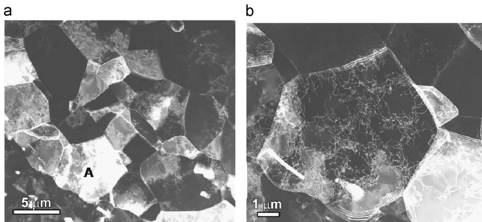
Fig. 5. TEM micrographs of the as-received 1100-O aluminum (a) and a magnified view of the grain labeled A (b).
