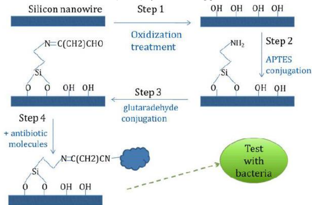
Figure 10, Schematic diagram of SiNWs modification
