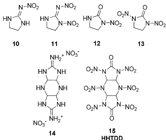
Figure 5. Literature examples of substrates believed to extrude \text{N}_2\text{O} .
