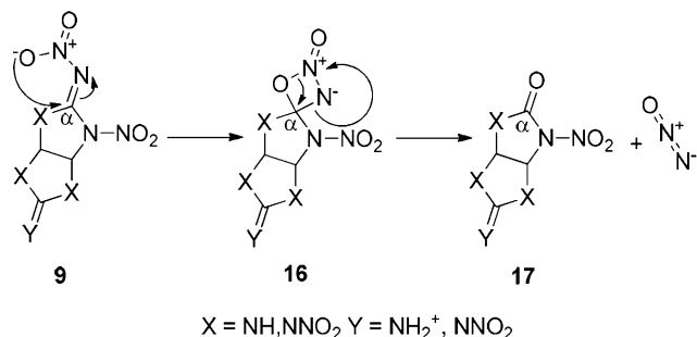
Scheme 1. Proposed mechanism for the intramolecular decomposition and extrusion of \text{N}_2\text{O} .
