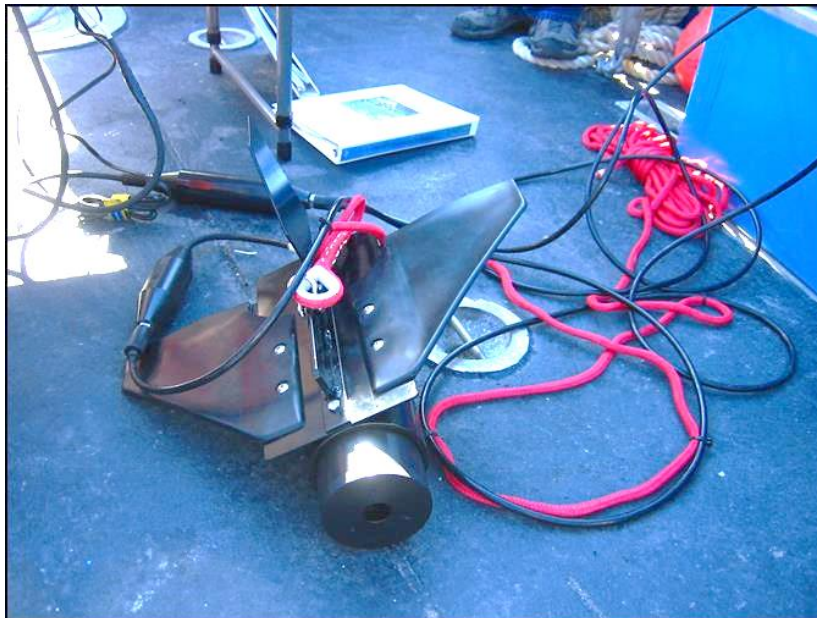
Figure C-23. Turner Designs C3 Fluorometer with tow package ready for deployment.
