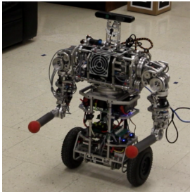
Figure 1.3 The uBot-5 mobile manipulator.
