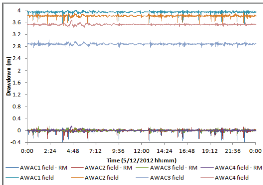
Figure 24. Raw depth field data and depth field data with removed mean (RM).
