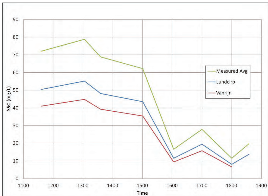
Figure 48. Range 4 SSC measured values and model estimates.
