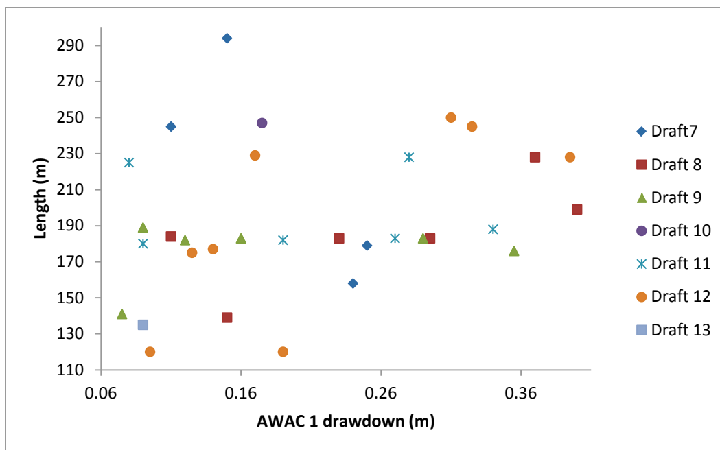
Figure 101. Drawdown at AWAC 1 vs. length for drafts 7–13 m.
