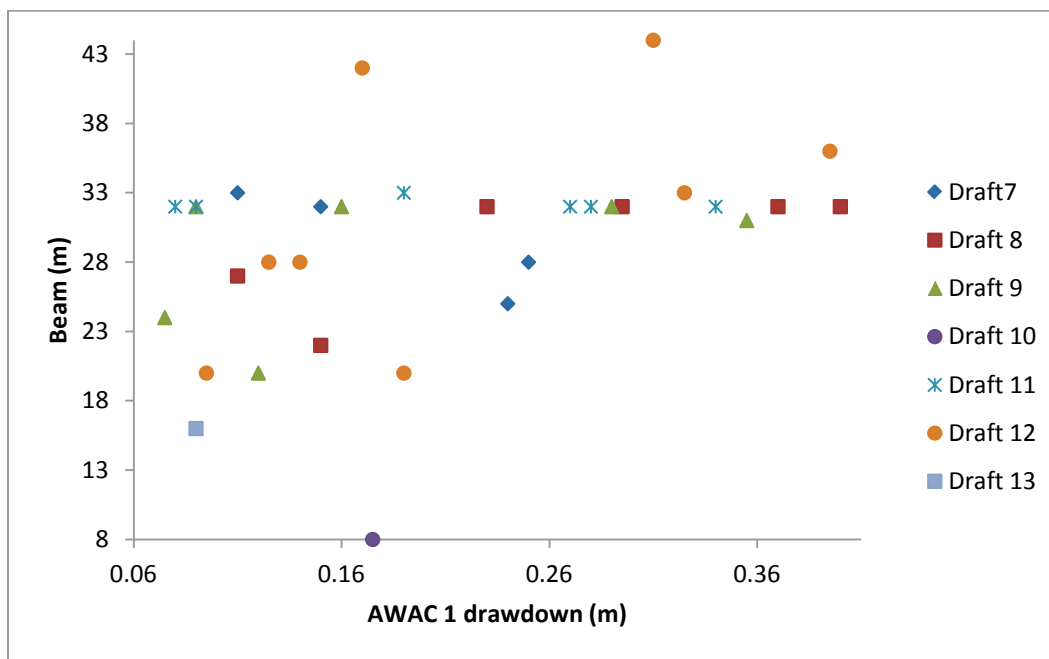
Figure 100. Drawdown at AWAC 1 versus beam for drafts 7–13 m.
