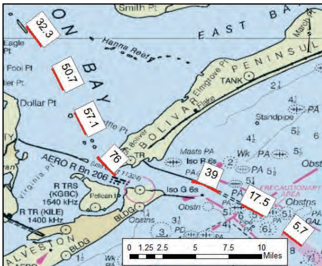
Figure 84. Percent sand measured in the navigation channel.
