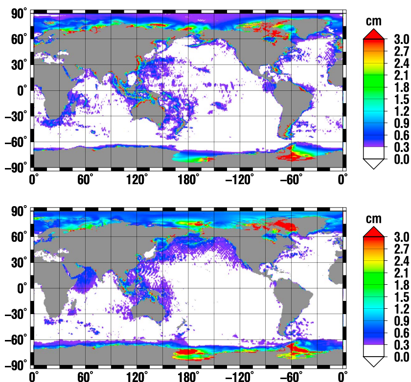
Figure 1. Standard deviations for (top) M_2 and (bottom) K_1 from the seven modern data-constrained models listed in Table 1.
