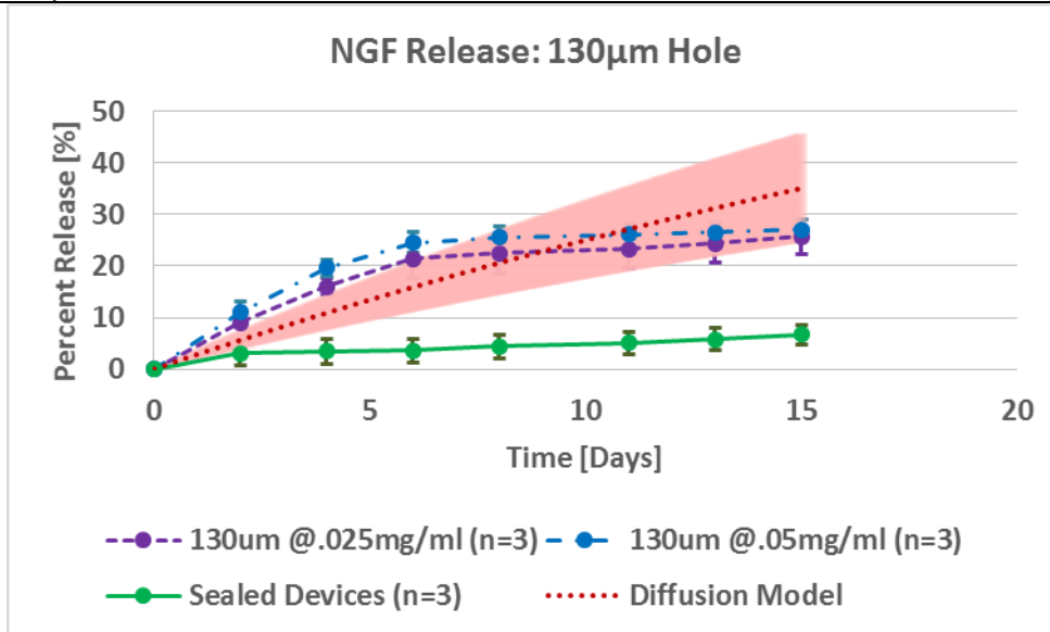
Figure 8 Release data for NGF with single 130 μm hole. The device is an all PLGA with inner conduit and PLGA drug reservoir. A CO 2 laser is used to create diffusion hole in PLGA conduit. No filter membrane is used for this device thus simplifying manufacturing.
