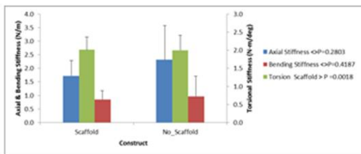
Figure 3. Axial, bending, and torsional stiffness for with and without scaffold. Error bars denote 1 standard deviation.
