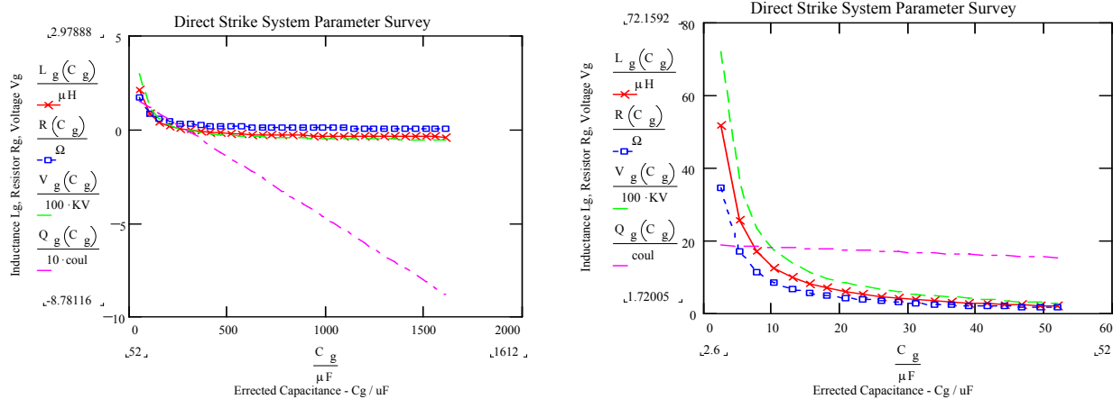
Figure 1. DSLTF Overdamped Parameter Surveys based on the off-shelf capacitor designs of G.A. Energy Products [5.B] . Note: beyond 260 μF, the iterated L_g becomes negative and should not be considered, else reducing R - L_g - C_g loop ( h , l ) to impractical small size \ll 30'' \times 3'' .
