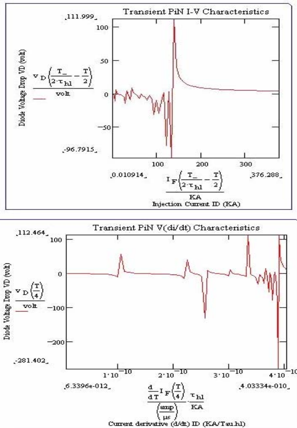
Figure 4.B MATHCAD Simulations for Transient I-V Characteristics and V_{frr} vs di/dt .
