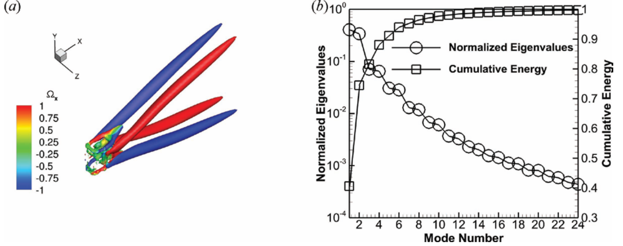
Figure 43. (a) Iso-surface of the Q -criterion of mean vorticity colored by the X-direction vorticity \bar{\omega}_x . Q=0.25 ; (b) Normalized eigenvalues (circle) and captured energy by the first i modes (square) versus mode number i=1, 2, \dots, 24 .
