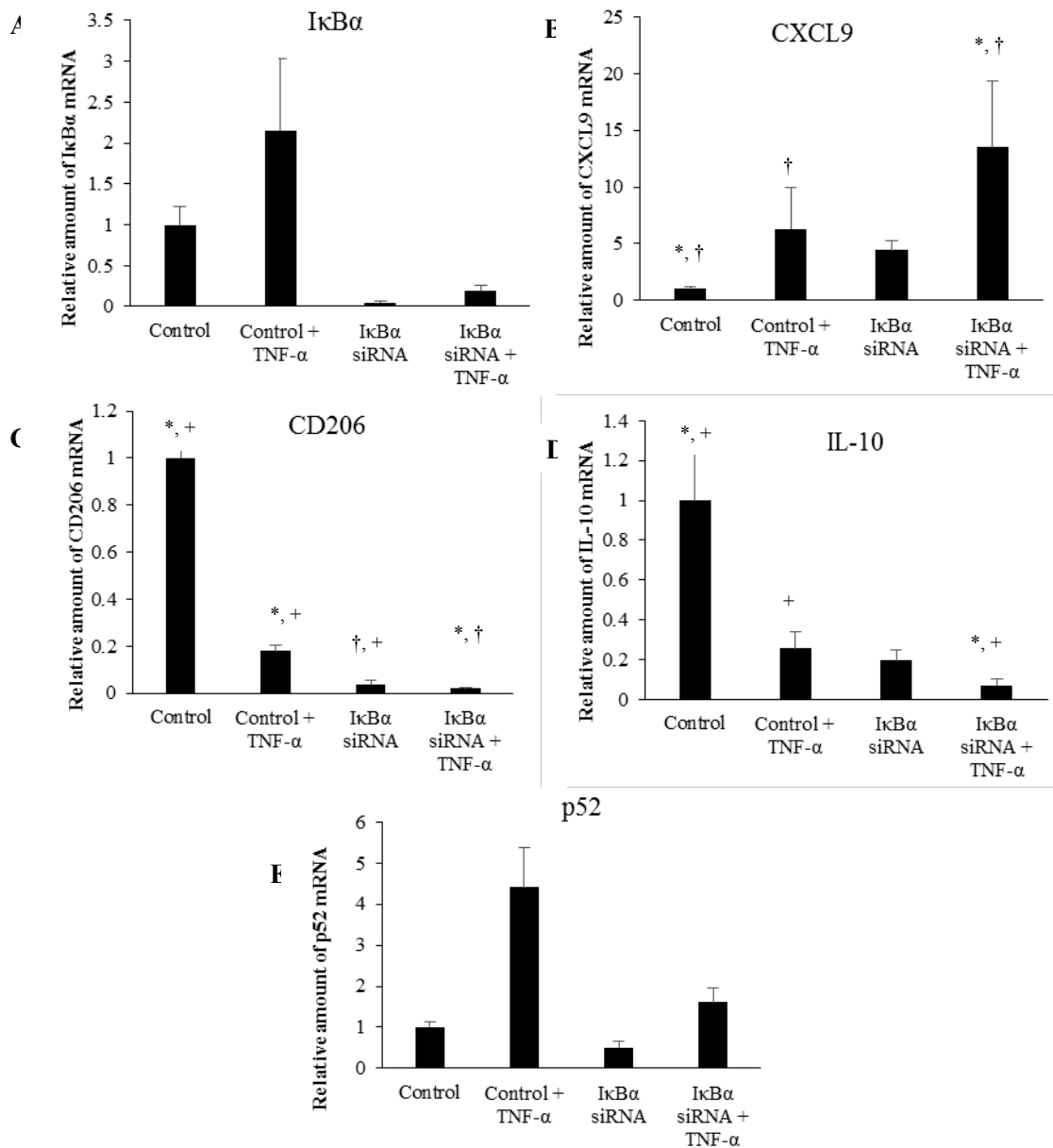
Figure 4: qRT-PCR of IκBα siRNA transfected BMDMs. (A) IκBα siRNA significantly knocks down IκBα mRNA. Although stimulation with TNF-α increase IκBα mRNA, this effect is significantly reduced by IκBα siRNA. (B) IκBα siRNA increases mRNA for T-cell recruitment cytokine, CXCL9. The increase in CXCL9 mRNA by transfection alone is not significantly different than the increase caused by TNF-α alone. (C) IκBα siRNA decreases mRNA for the mannose receptor, CD206, a trophic, TAM phenotypic marker. TNF-α alone and MnNP delivered siRNA alone cause a significant decrease in CD206 mRNA. The combination of the two results in significantly greater decrease in CD206 mRNA. (D) IκBα siRNA decreases mRNA for IL-10, an immunosuppressive cytokine. The decrease in IL-10 mRNA by transfection alone is not significantly different than the decrease caused by TNF-α alone, but the combination of the two results in less IL-10 mRNA than either condition by itself. (E) IκBα siRNA decreases mRNA for p52. As previously shown, TNF-α stimulation of macrophages increases levels of p52 mRNA, indicating that p52 is a viable target for mRNA level knockdown. Transfection with IκBα siRNA reduces the increase in p52 mRNA caused by TNF-α, indicating potentially beneficial cross-talk between the two pathways which could be leveraged to act synergistically toward altering the TAM phenotype to an anti-tumor phenotype. † : P ≤ 0.01, *, + : P ≤ 0.005
