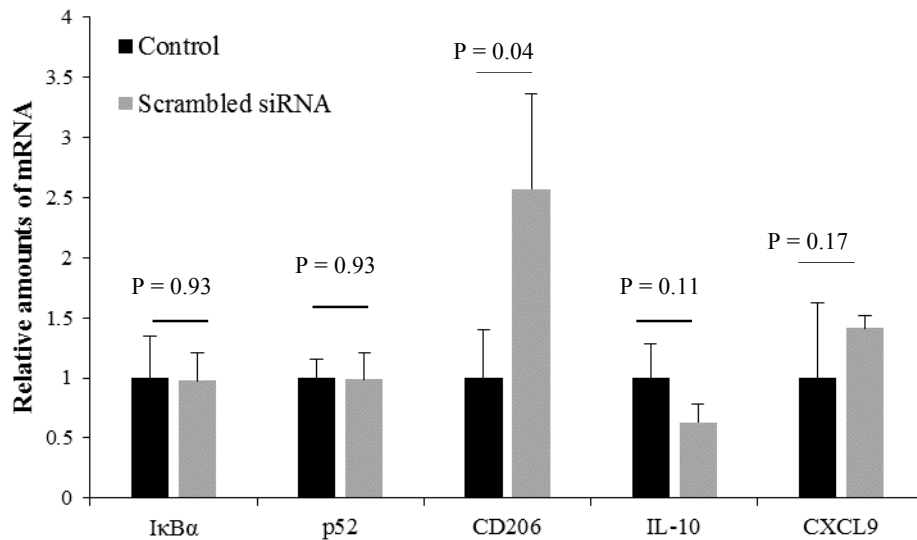
Figure 5: qRT-PCR of scrambled siRNA transfected BMDMs. There is no significant decrease in mRNA levels between the two groups for IkBα, p52, IL-10 and CXCL9. There is a significant increase in CD206 mRNA following culture with MnNP loaded with a scrambled siRNA sequence. This is consistent with previous reports that activation and endosomal transport of the mannose receptor increases mannose receptor production in macrophages.
