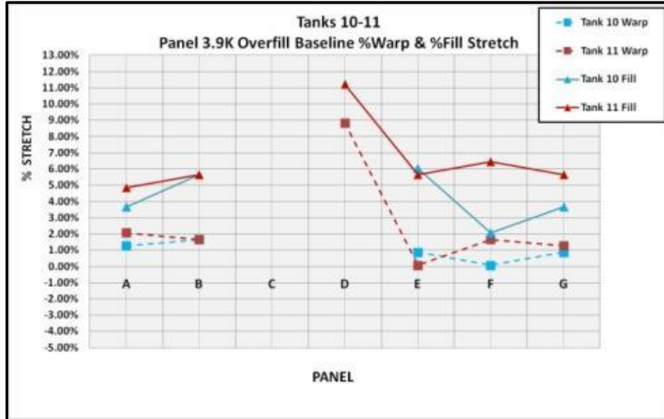
Figure 5.4.6 – Tank 10/11 3.9K Overfill Stretch Measurements
