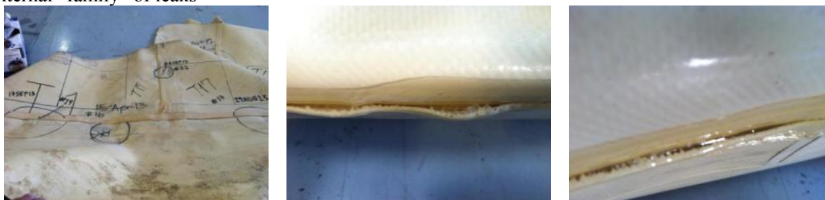
Figure 5.4.109 – Class I – T17-19,16,17 – Closing Seam – 3 JUL, 19 AUG, 17SEP 13 Gaps between material panels encased in adhesive – example of single internal root cause for multiple external “family” of leaks
