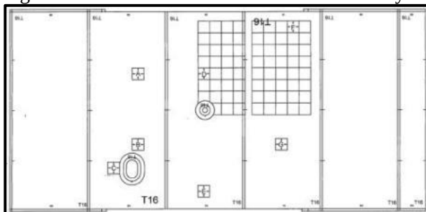
Figure 5.4.15 – Tank 16 Measurement Panel Layout
