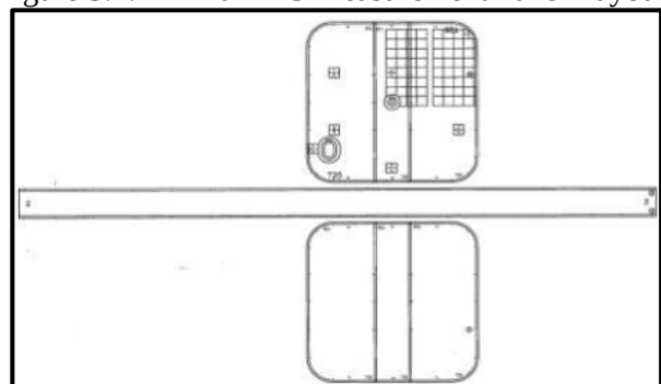
Figure 5.4.24 – Tank 25 Measurement Panel Layout
