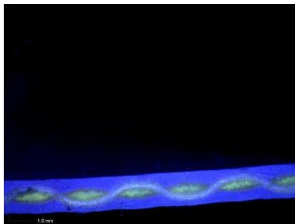
Figure 6.2.35 – Single butt seam weld (1) – top butt seam showing limited dye penetration down center from exposed end ; dye intensity drops moving outward in the butt seam. Bottom panels showing some limited penetration from open interior face (2).
