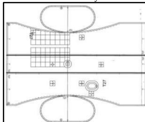
Figure 5.4.26 – Tank 27 Measurement Panel Layout
