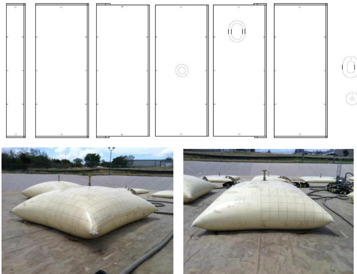
Figure 4.4.16 – Typical Standard Design tank showing elevated corners and ends
