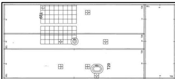
Figure 5.4.28 – Tank 29 Measurement Panel Layout
