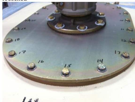
Figure 6.2.102 – Tank fitting with bolts 12-19 loosened
