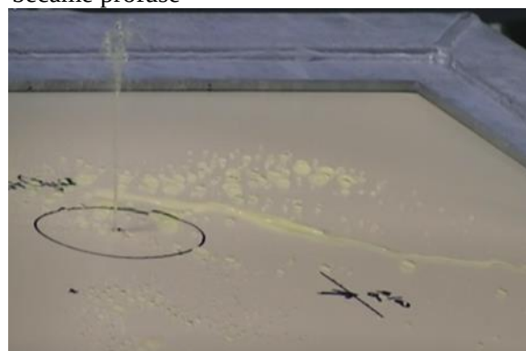
Figure 6.2.70 – At pressure of 15 in H 2 O, leak became profuse
