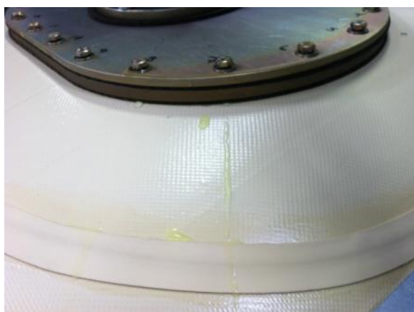
Figure 6.2.96 – Dye penetration in material scrim for bolt-hole 7
