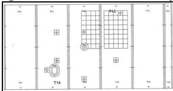
Figure 5.4.11 – Tank 14 Measurement Panel Layout
