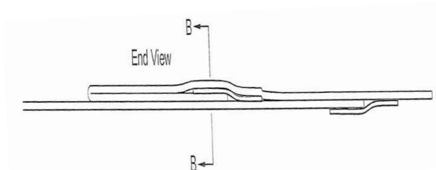
Figure 4.2.7 – Fold-Over Prayer Weld Closing Seam
