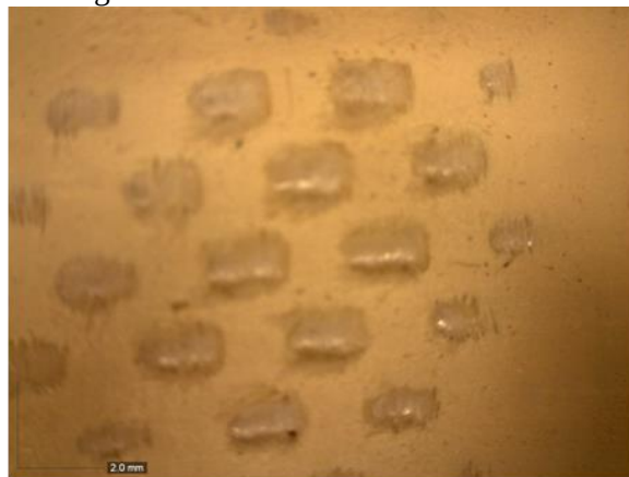
Figure 6.2.58– View of FCF2-4 scuffs with dye seeping (FCF2) and weeping (FCF3-4)
