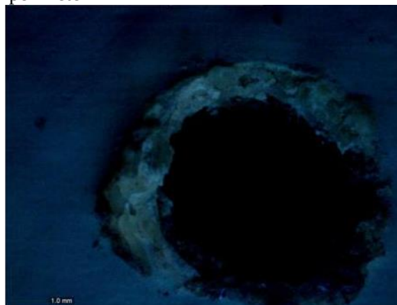
Figure 6.2.95 – Bolt-hole 7 under black light with slight dye penetration in scrim around perimeter
