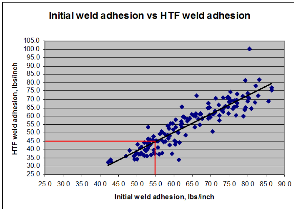
Figure 6.1.1 – Initial Weld and HTF Load Correlation
