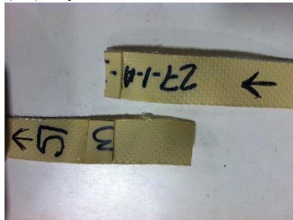
Figure 6.1.9 – Torn Inside Weld (TIW) sample
