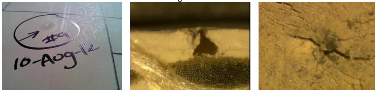
Figure 5.4.87 – Class I – T17-9 – Panel – 10 AUG 12 Potential external contamination based on cracking and discoloration near surface
