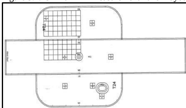
Figure 5.4.23 – Tank 24 Measurement Panel Layout
