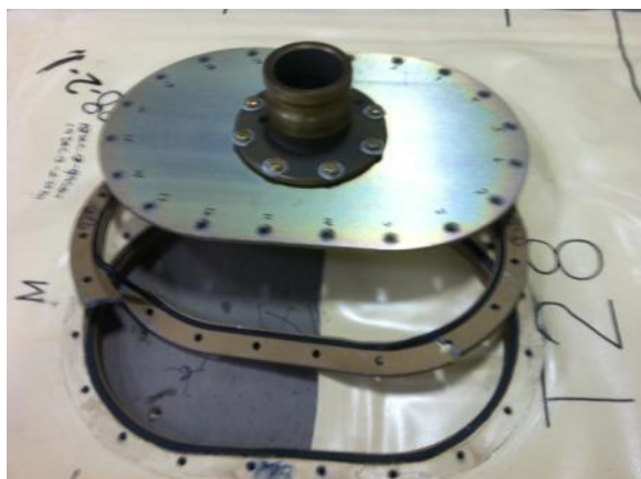
Figure 6.2.99 – Tank 28 O-ring compression exploded fitting stack-up
