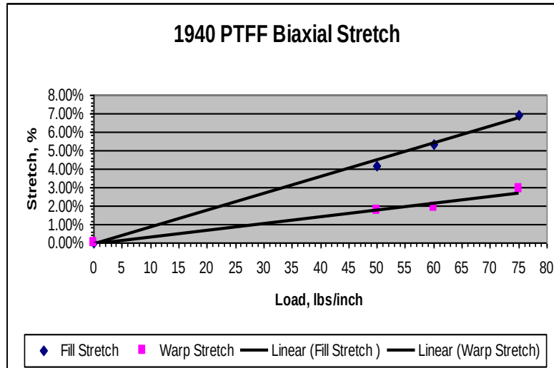
Figure 4.2.10 – 1940 PTFE Biaxial Stretch Curve
