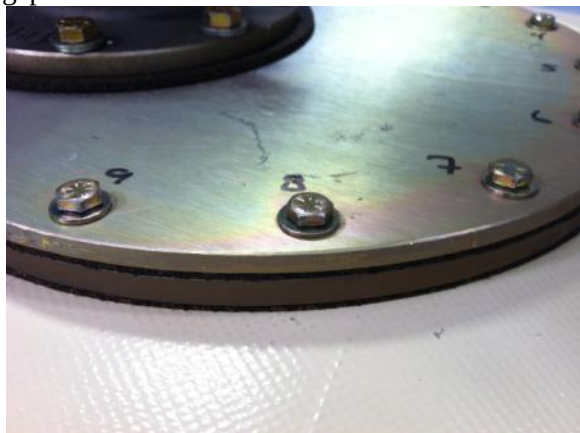
Figure 6.2.92 – Bolts 7-9 loosened with a 1 mm gap
