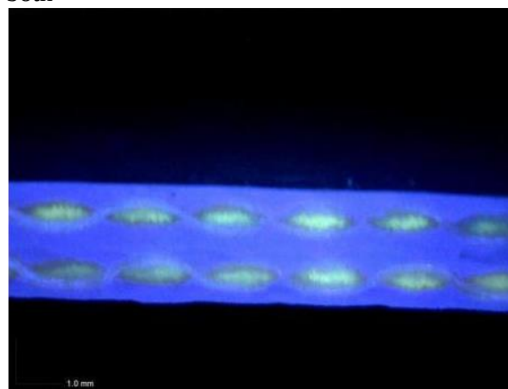
Figure 6.2.33 – Shingle overlap weld with two interior scrim exposed panels – dye penetration in both
