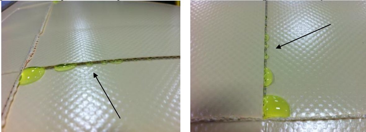
Figure 6.2.12 – Perpendicular and parallel views of SO outer seam showing individual droplet formation
