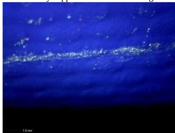
Figure 6.2.40 – Internal overlap weld seam – residual dye apparent in weld seam edge
