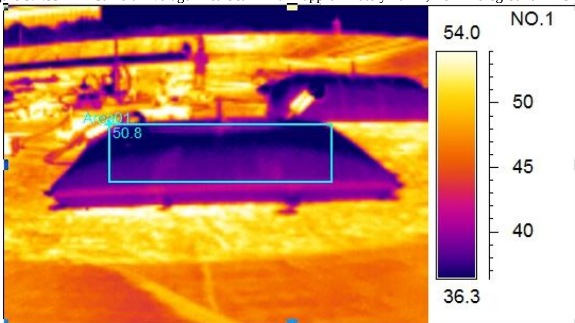
Figure 5.4.59 – IR Camera Average Area Scan – Tank approximately 101°F, Berm Foreground ~125°F
