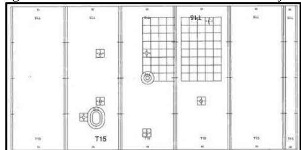
Figure 5.4.12 – Tank 15 Measurement Panel Layout
