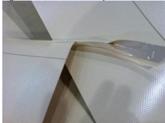
Figure 4.5.10 – 2” Weld Completion
