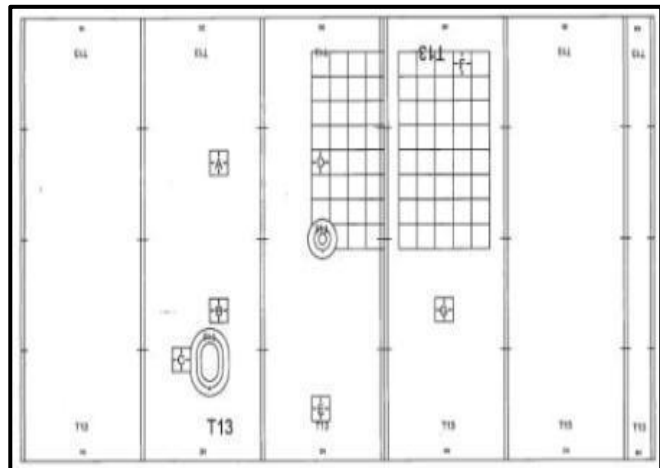
Figure 5.4.8 – Tank 13 Measurement Panel Layout
