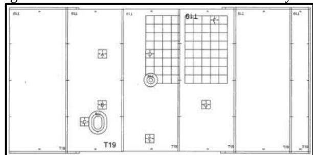
Figure 5.4.16 – Tank 19 Measurement Panel Layout
