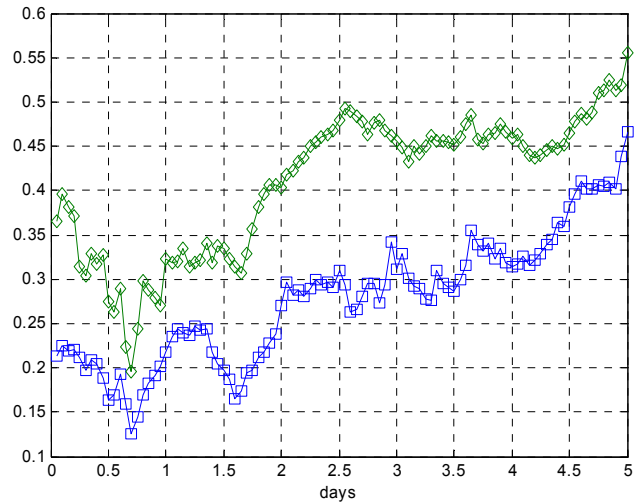
Figure 2. Relative error of interpolation for the suggested OI (blue) and the simplest one (Molcard et al,2003)
