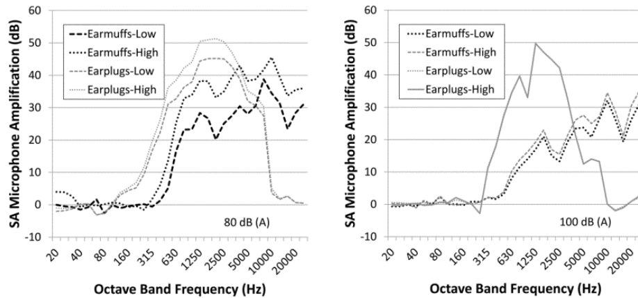
Fig. 9 SA microphone amplification as measured at 0° for each of the ambient noise conditions
