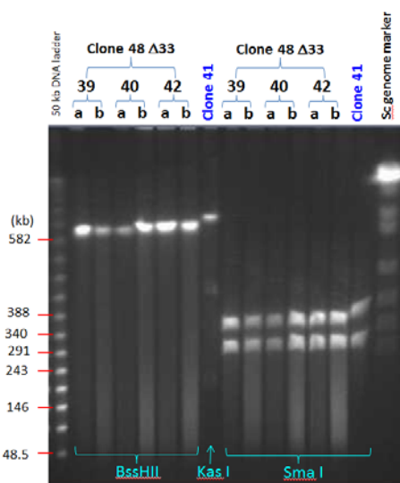
Figure 9. Restriction analysis of Cluster 33 deletion from Clone 48.
