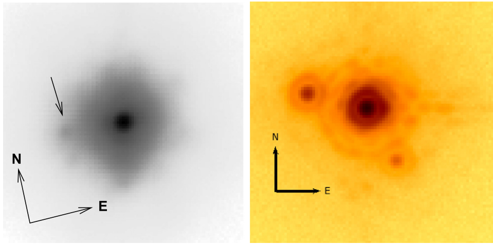
Figure 4. On the left is an i image of 30 Ari BC from Robo-AO. It is a subimage of the full 44'' field of view and is \sim 2''5 across. The location of the newly discovered companion is indicated by the arrow. On the right is a K_s image of 30 Ari BC acquired with the PALM 3000 AO system. The object to the lower right of the primary star of the image is a ghost image caused by the neutral density filter. This is a subimage of the full 25'' field of view and is \sim 2'' across.
