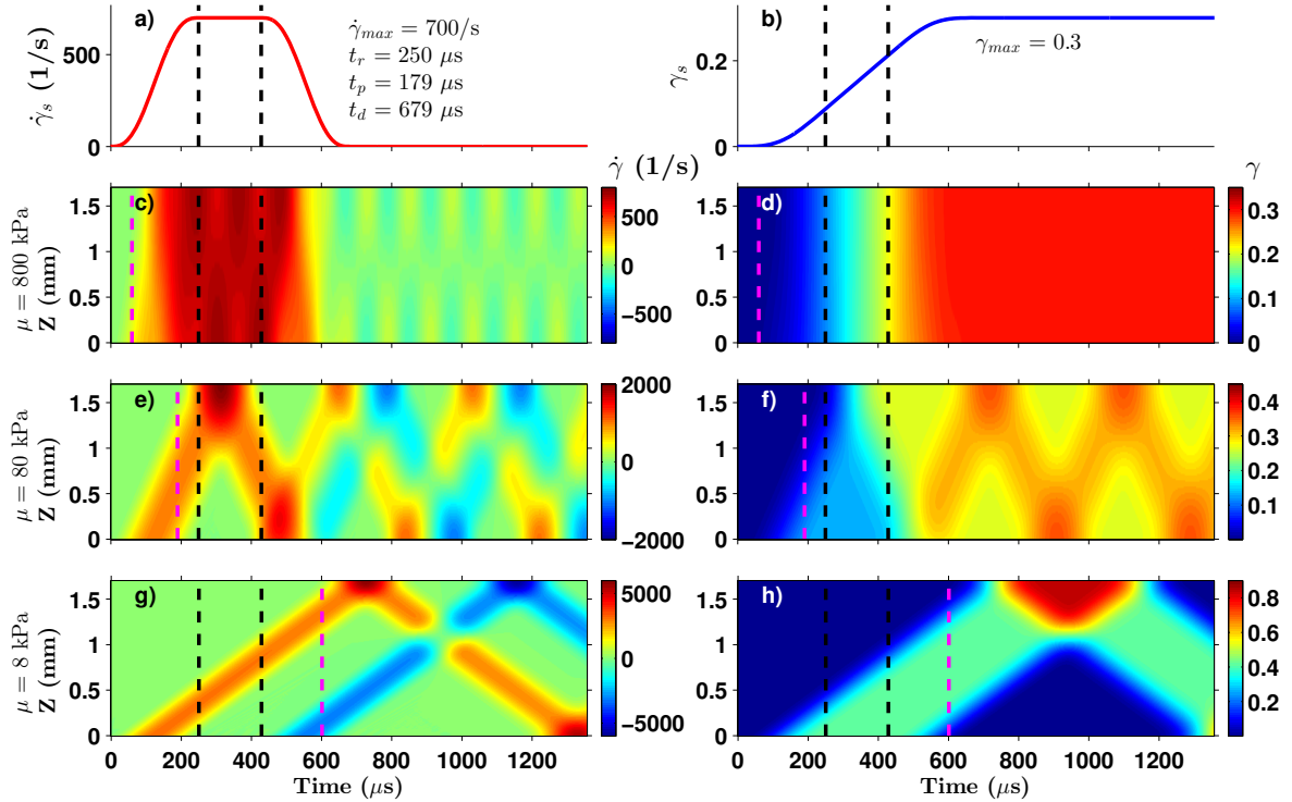
Figure 3. The average strain-rate history \dot{\gamma}_s(t) (panel a ) and corresponding average strain history \gamma_s(t) (panel b ) imposed on the specimen for Simulations I–III . The first black vertical dashed line corresponds to the rise time t_r to constant strain-rate. The second black vertical dashed line is the time ( t_r + t_p ) at which the strain-rate starts to ramp down after a constant strain-rate plateau of duration t_p . The remaining panel pairs ( c–d , e–f , and g–h ) are false color images of the corresponding actual strain-rates \dot{\gamma}(z, t) and strains \gamma(z, t) in specimens with shear moduli \mu = 800 , 80, and 8 kPa, respectively. Note that the color scale varies for the three groups of plots. The vertical magenta lines correspond to t_{travel} , which depends on the shear modulus.
