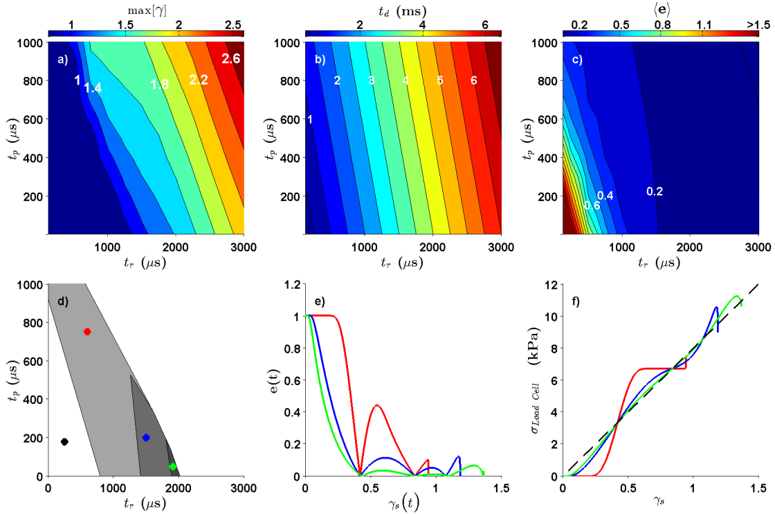
Figure 5. Panels a – c show the effects of varying the rise time t_r (horizontal axis) and the plateau time t_p (vertical axis) for \dot{\gamma}_{\max} = 700/\text{s} tests on a linear elastic specimen with shear modulus 8 kPa. Through false-color images, these panels show the peak strain reached at the Load Cell during a simulation ( \max[\gamma] , panel a ), the total loading pulse duration t_d (panel b ), and the average error \langle e \rangle in the strain (see text, panel c ). Panel d shows the regions where the peak strain is less than 1.5, the total pulse duration less than 5 ms, and the average error less than 40%, 20%, and 15% in darkening shades of gray. The black dot represents Simulation III , which most closely resembles the test conditions in [Nie et al. 2013]. The red, blue, and green circles are sample test conditions taken in each region. Additional results for these test conditions are given in panels e and f . Panel e is a plot of e(t) (the relative error in the strain at the Load Cell ) versus the average imposed strain \gamma_s(t) . Panel f shows the resultant stress-strain curves. The black dashed line represents the ideal to which these curves should be compared, that is, the curve that would have been produced if \gamma_s(t) coincided with \gamma_{\text{Load Cell}} .
