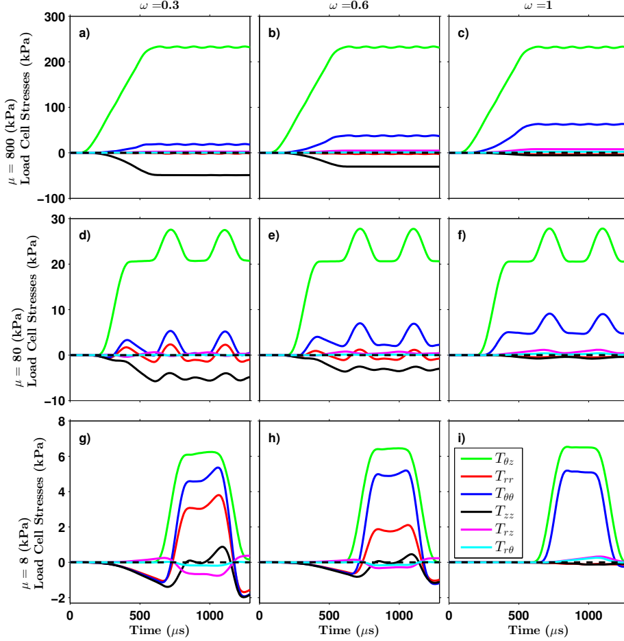
Figure 7. The radially averaged stress components at the Load Cell ( Z = L ) versus time for the nine simulations: two decades of shear modulus ( \mu = 800, 80 , and 8 kPa) and three values of dimensionless parameter ( \omega = 0.3, 0.6 , and 1.0 ). All simulations used the same 700/\text{s} loading pulse as the one-dimensional Simulations I–III ; see Table 2 and panels a and b in Figure 3. The legend for the line colors is given in panel i and is consistent throughout the figure. Note the change in vertical scales for the different rows.
