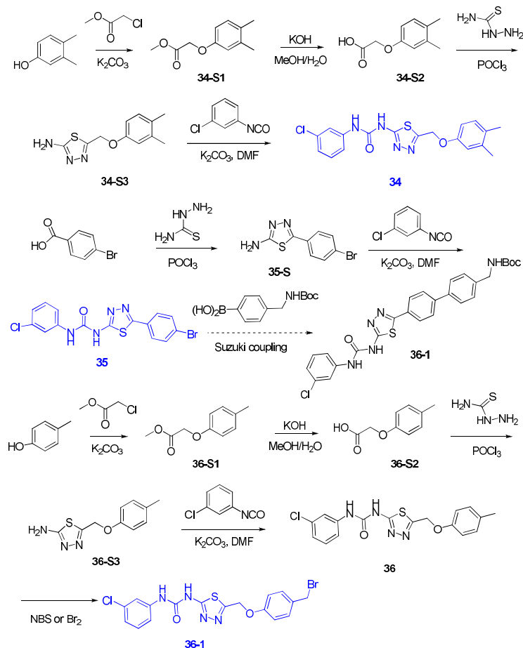
Scheme 8. Synthesis of hepsin-binding ligands with a diarylurea
