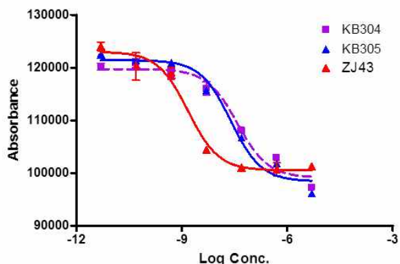
Fig. 8. IC 50 curves of KB304-KB305
