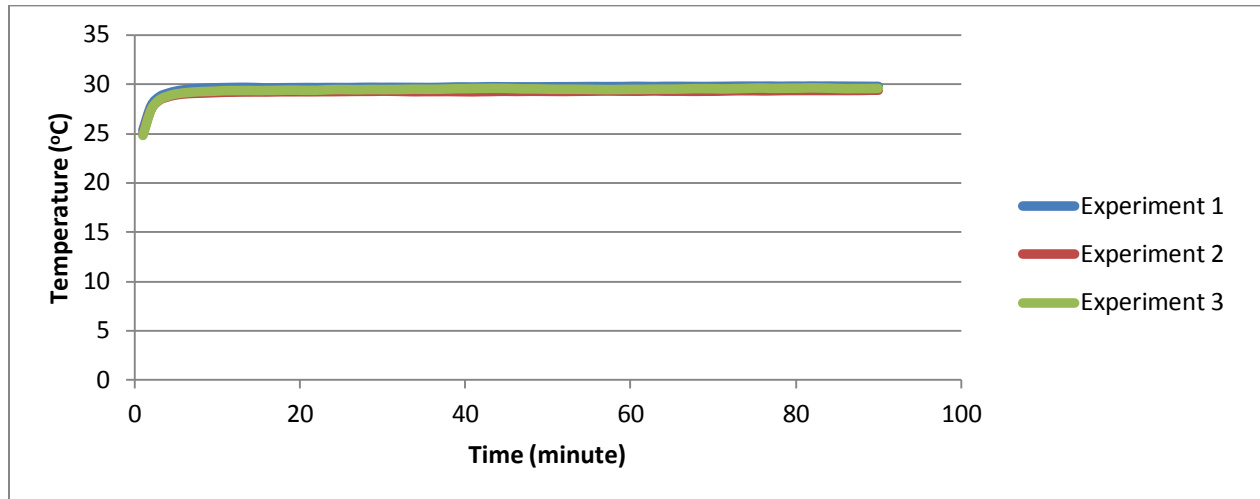
Figure 58. Comparison of body average skin temperature of thermal manikin in neutral (25°C) ambient conditions
