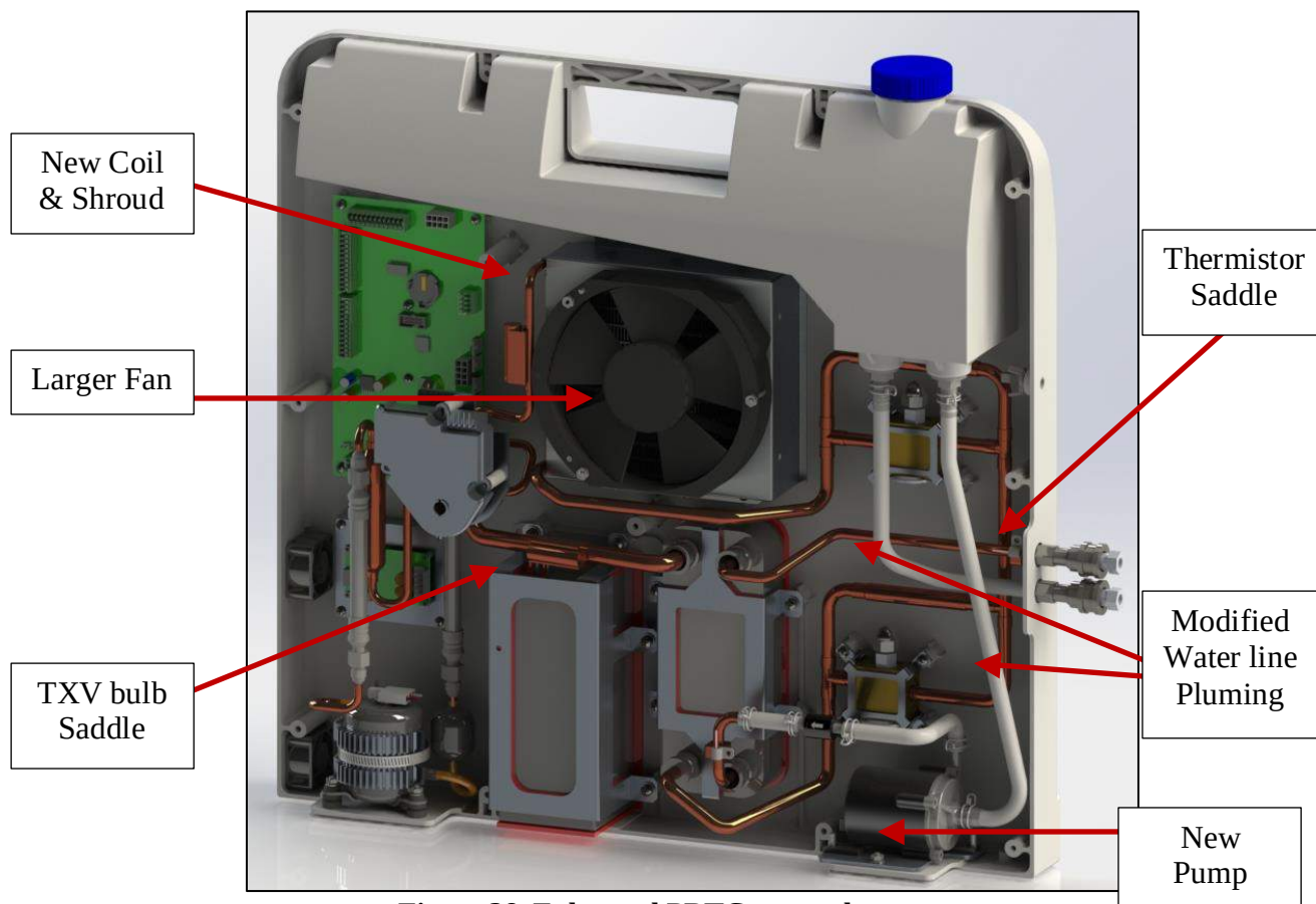
Figure 28. Enhanced PBTC system layout
