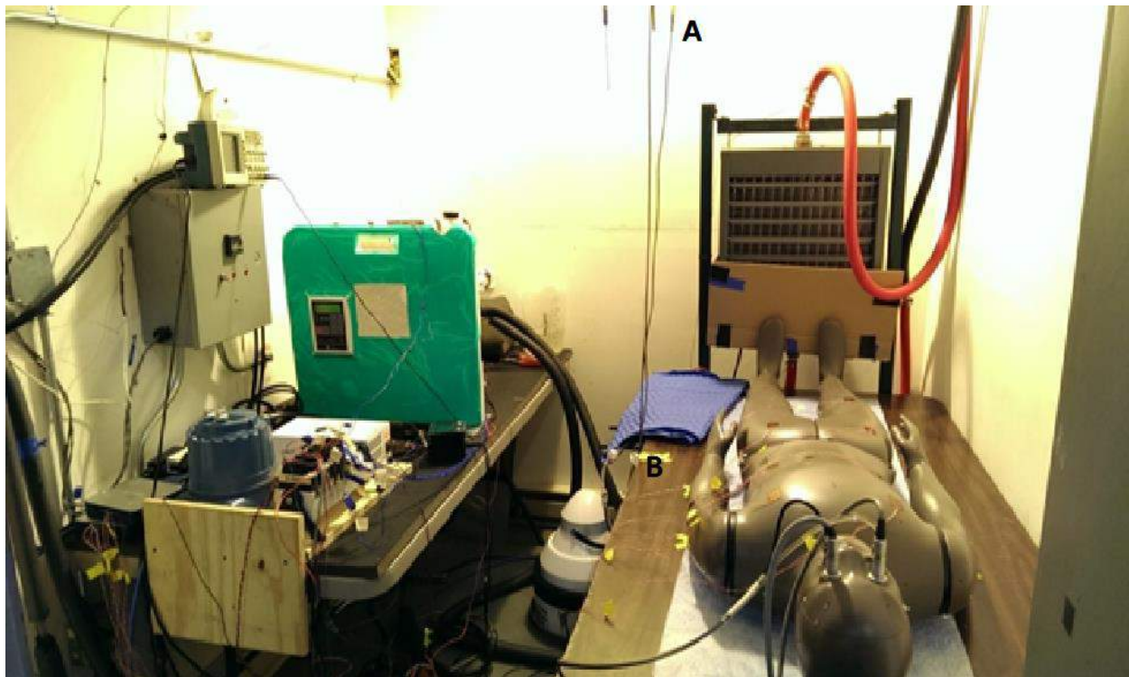
Figure 67. Environmental chamber at Rocky Research
