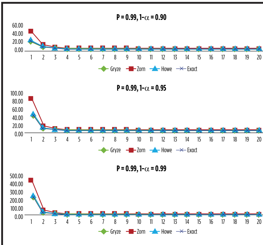
FIGURE 2. P = 0.99, 1-\alpha = \{0.90, 0.95, 0.99\}
