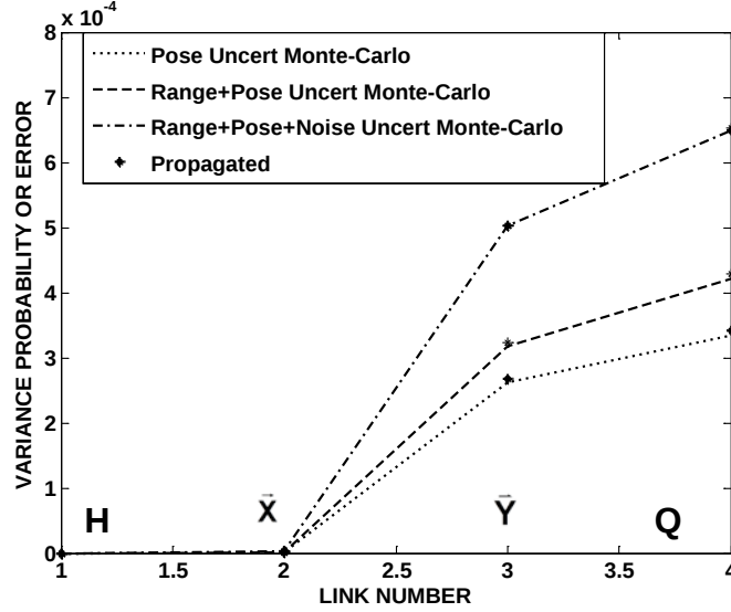
Fig. 25. Reliability in Predicted Link Performance Given as Variance, L=50 , N=3*105
