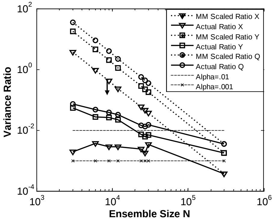
Fig. 18. Sampling Uncertainty and Testing N_M at \bar{X} , \bar{Y} , Q
