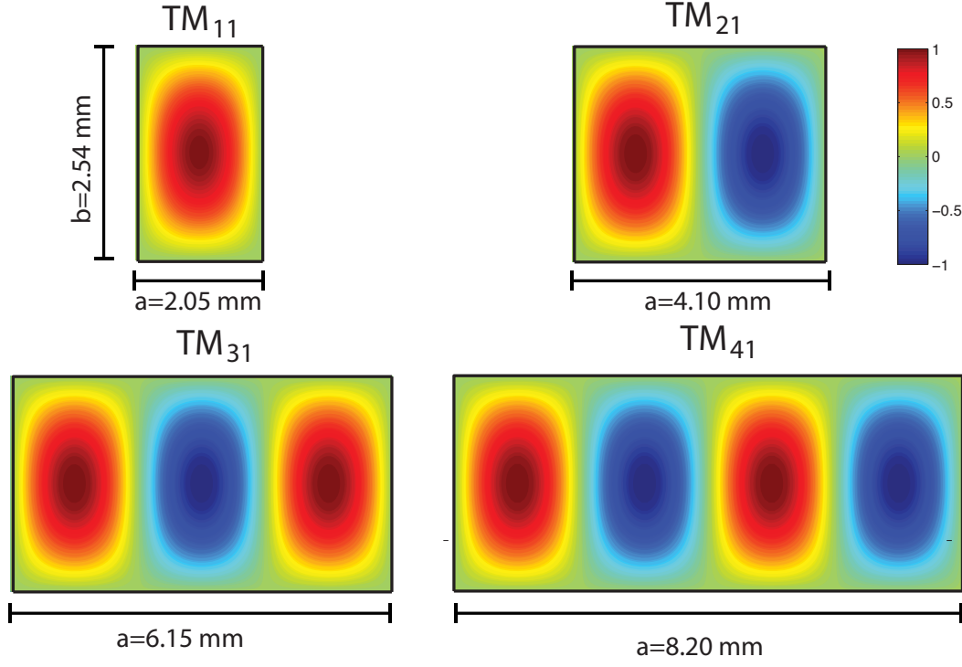
Figure 3-2: Contour plots of the electric field, E = E_z , for some of the lowest order cavity modes. For each mode, b has been set to 2.54 mm, and a is determined such that the mode will oscillate at 94 GHz.
