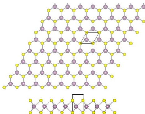
Figure 1 Top and side views of molybdenum disulfide ( MoS_2 ) (2H-polytype)
