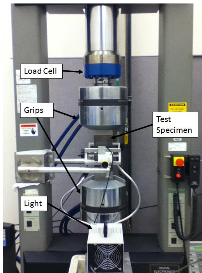
Fig. 7 Load Frame Equipment
