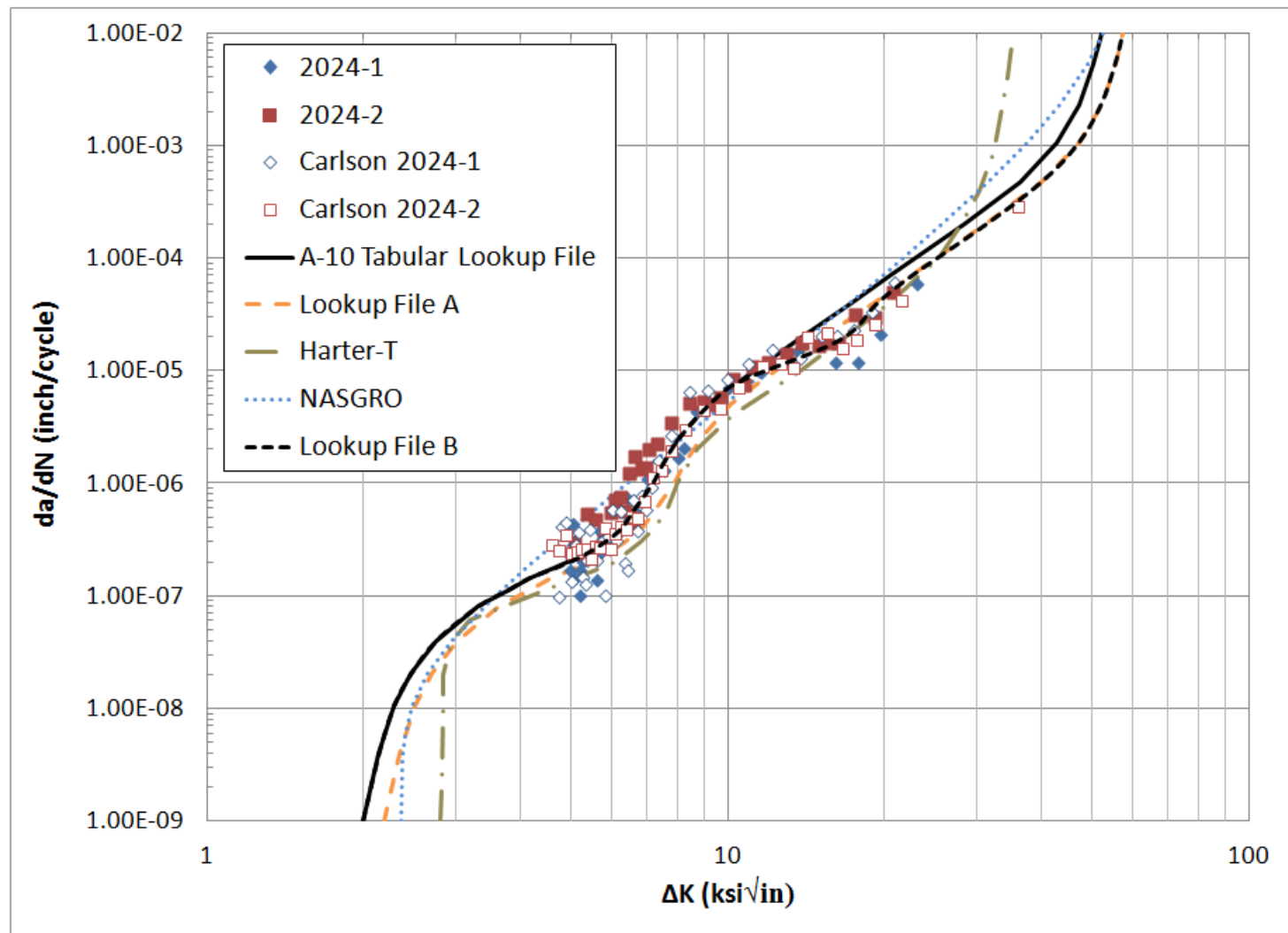
Fig. 91 da/dN vs. \Delta K Data and Common Curve Fits
